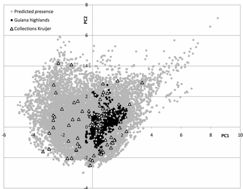
Fig. 11. Result of the PCA for the seven variables that explained more than 2.5% of the Maxent model based on Kruijer's data for those grid cells where H. tamarisci was predicted to be present (10 percentile threshold). Black dots indicate the Guiana Highlands. Triangles indicate collection localities.
