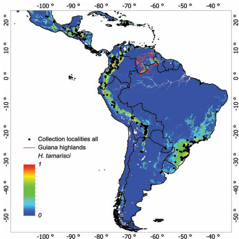
Fig. 3. Maxent distribution model for H. tamarisci based on 313 records from Kruijer and GBIF (see text). Probability of presence increases from dark blue (0) to red (1). Most areas in red are obscured by the black dots representing the collection localities. The red demarcation line indicates the Guiana Highlands (above 250 m asl).
