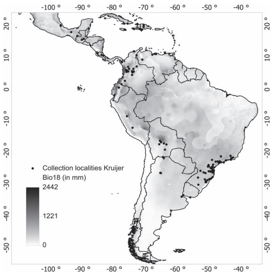
Fig. 7. The collection localities of the 125 unique records of Kruijer's data plotted on the bioclimatic variable Bio18 - Precipitation of warmest quarter (in mm). Darker grey tones indicate higher precipitation.
