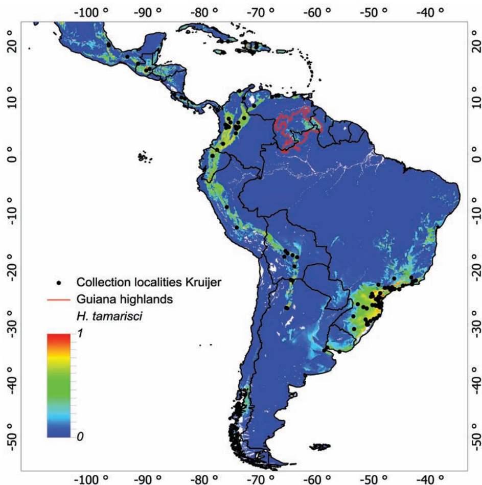
Fig. 1. Maxent distribution model for H. tamarisci based on 125 records from specimens identified by Kruijer (see text). Probability of presence increases from dark blue (0) to red (1). Most areas in red are obscured by the black dots representing the collection localities. The red demarcation line indicates the Guiana Highlands (above 250 m asl).
