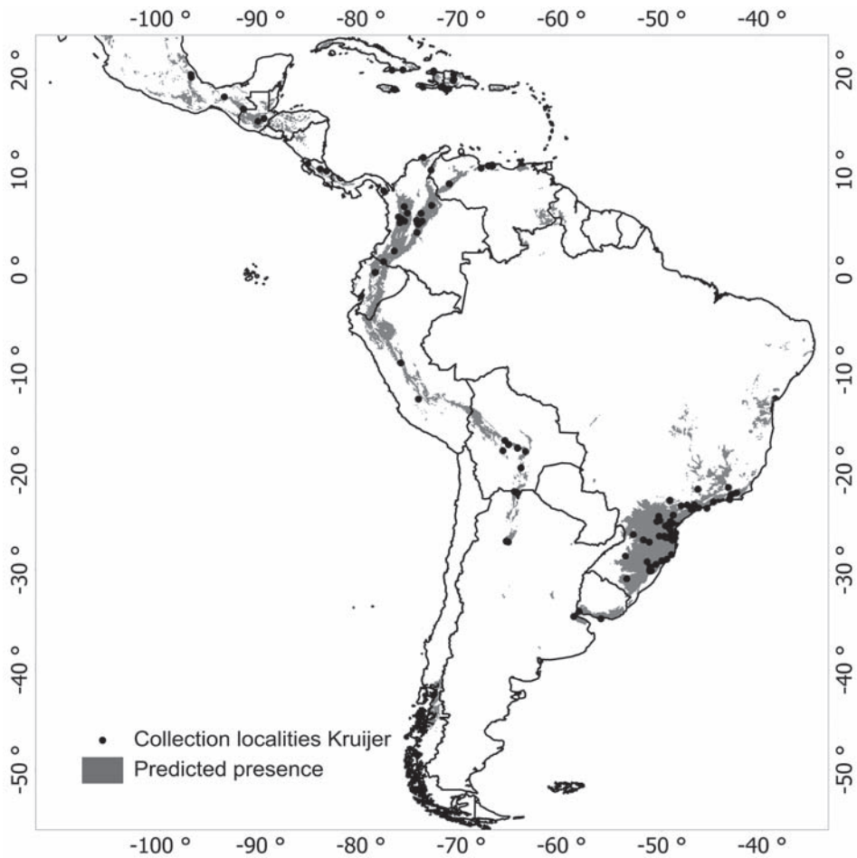
Fig. 2. Thresholded Maxent distribution model for H. tamarisci based on 125 records from specimens identified by Kruijer (see text). Grey areas indicate predicted presence.
