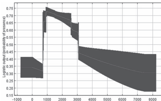
Fig. 10. The response curve for the bioclimatic variable Bio12 based on 10 times cross-validated Maxent models. This plot reflects the dependence of predicted probability of presence on Bio12. Bio12 contributes 10.6% to the full model.
