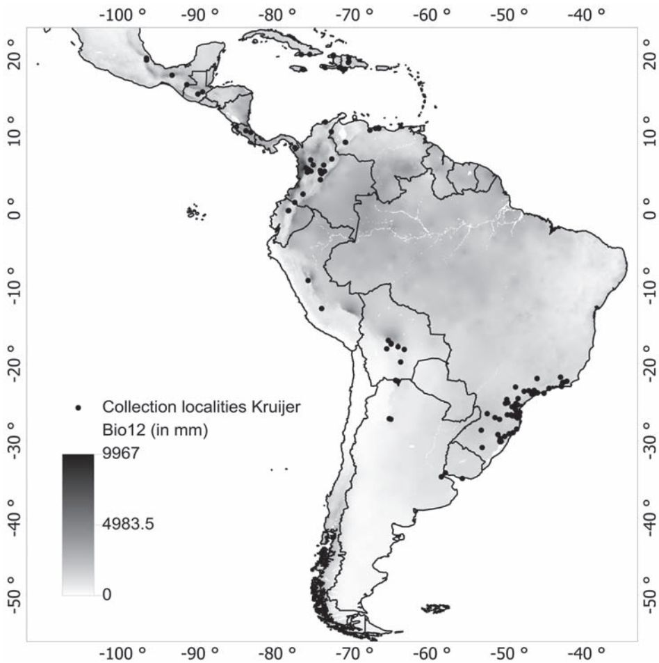
Fig. 9. The collection localities of the 125 unique records of Kruijer's data plotted on the bioclimatic variable Bio12 - Annual precipitation (in mm). Darker grey tones indicate higher precipitation.
