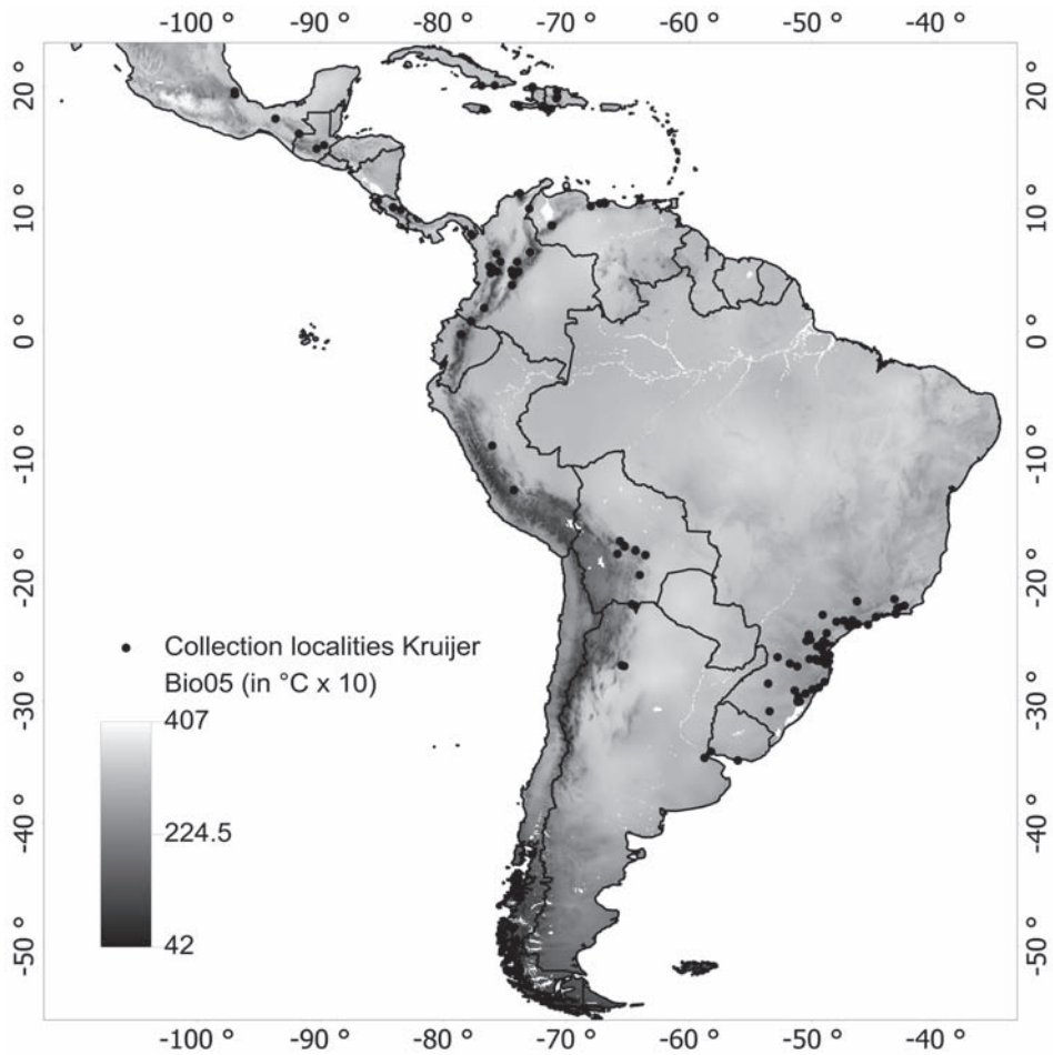
Fig. 5. The collection localities of the 125 unique records of Kruijer's data plotted on the bioclimatic variable Bio05 - Maximum temperature of warmest month (in °C × 10). Lighter grey tones indicate higher temperatures.
