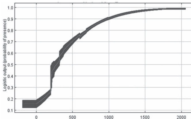
Fig. 8. The response curve for the bioclimatic variable Bio18 based on 10 times cross-validated Maxent models. This plot reflects the dependence of predicted probability of presence on Bio18. Bio18 contributes 16.4% to the full model.
