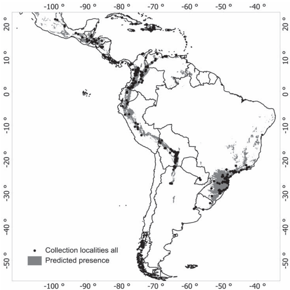
Fig. 4. Maxent distribution model for H. tamarisci based on 313 records from Kruijer and GBIF (see text). Grey areas indicate predicted presence.
