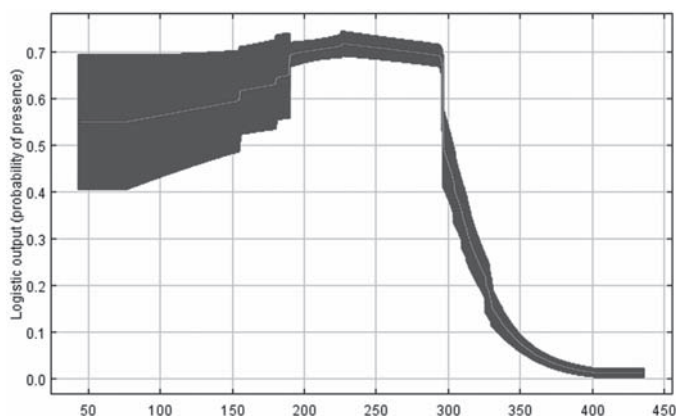
Fig. 6. The response curve for the bioclimatic variable Bio05 based on 10 times cross-validated Maxent models. This plot reflects the dependence of predicted probability of presence on Bio05. Bio05 contributes 43.9% to the full model.
