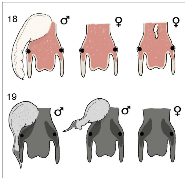
Figs 18–19. Anatomies of two valvatiform species of Hydrobiidae. 18. Kulyiella marginata gen. nov. spec. nov. Male showing the robust penis, broad at the base and tapering into a small apical papilla, and females, including one with a pseudopenis. 19. Ganduliella irrippensis gen. nov. spec. nov. Males showing the characteristic penis, strongly broadened at the base and tapering into a narrow neck-like portion with a brush-shaped apex.
