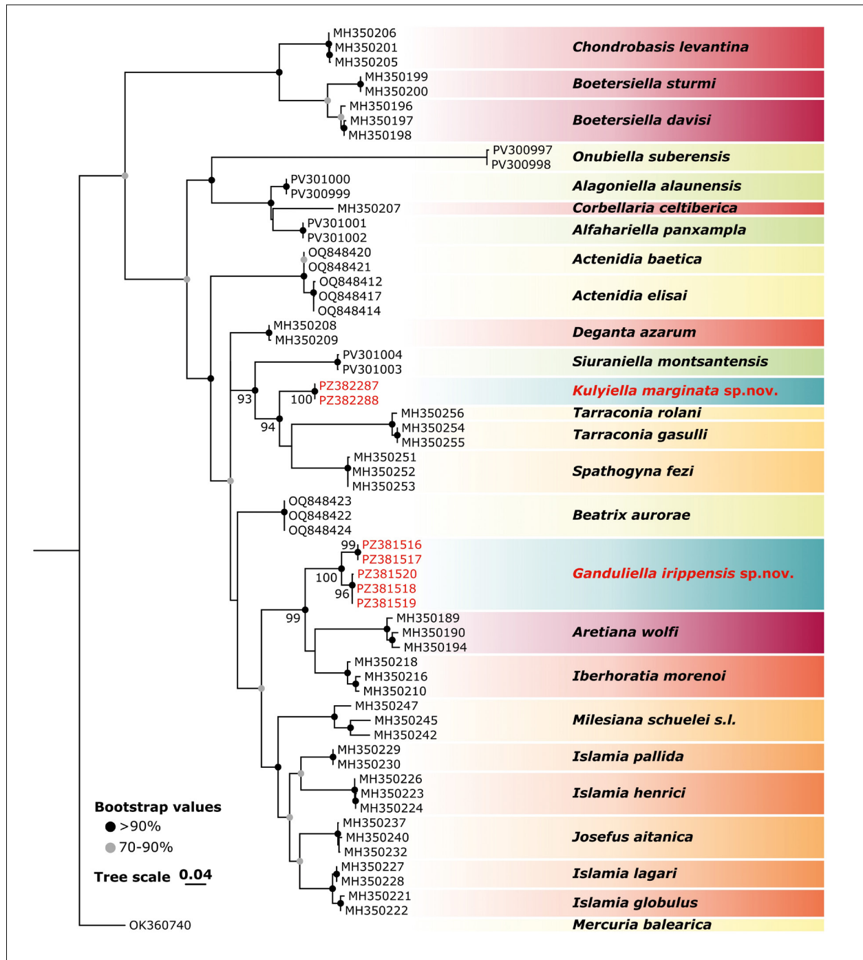
Fig. 17. Maximum likelihood phylogeny inferred using the COI dataset in IQ-TREE. Ultrafast bootstrap values are provided at relevant nodes. GenBank accession numbers are listed adjacent to each scientific name. Each color represents a different species. The new sequences are highlighted in red.
