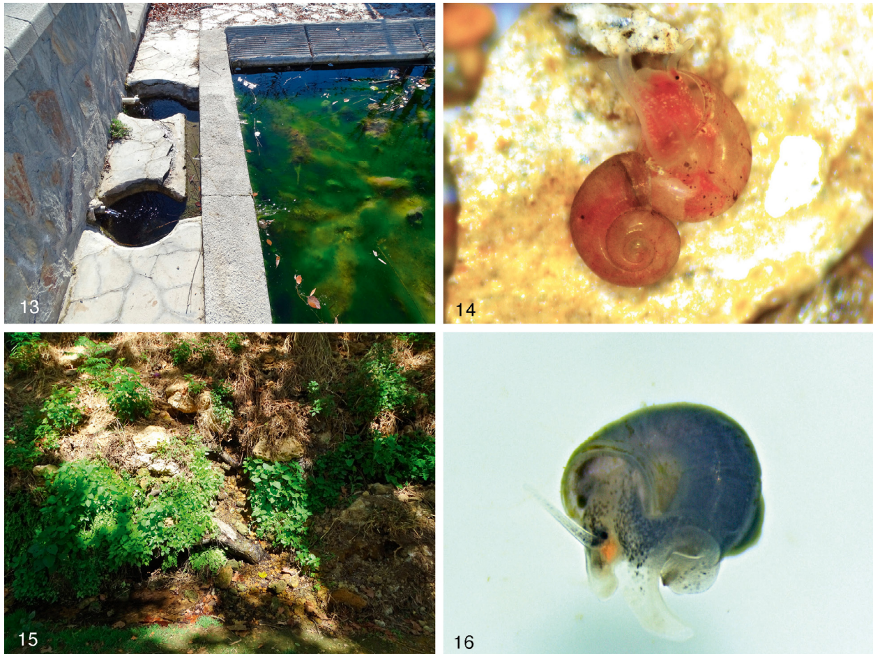
Figs 13-16. Type localities of the newly described species. 13-14. El Caño del Margen, El Margen-Cúllar (Granada province), type locality of Kulyiella marginata gen. nov. spec. nov. 15-16. Spring at Camino de la Huerta de la Peñuela, Alcalá de Guadaira (Sevilla province), type locality of Ganduliella irippensis gen. nov. spec. nov.
