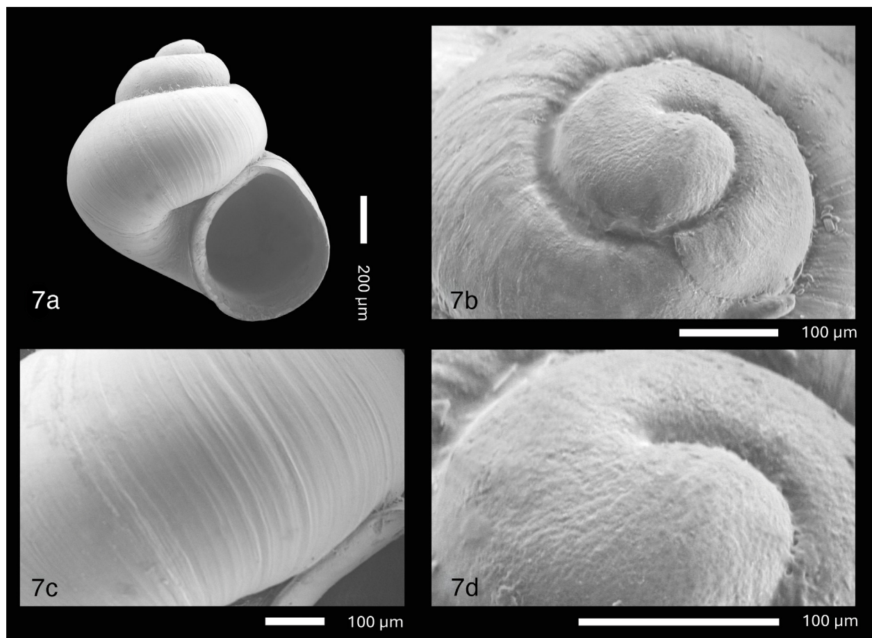
Fig. 7. SEM images of Ganduliella irippensis gen. nov. spec. nov. Different views of a paratype. 7a. Frontal view. 7b. Protoconch apical view. 7c. Detail of the teleoconch. 7d. Detail of the protoconch.
