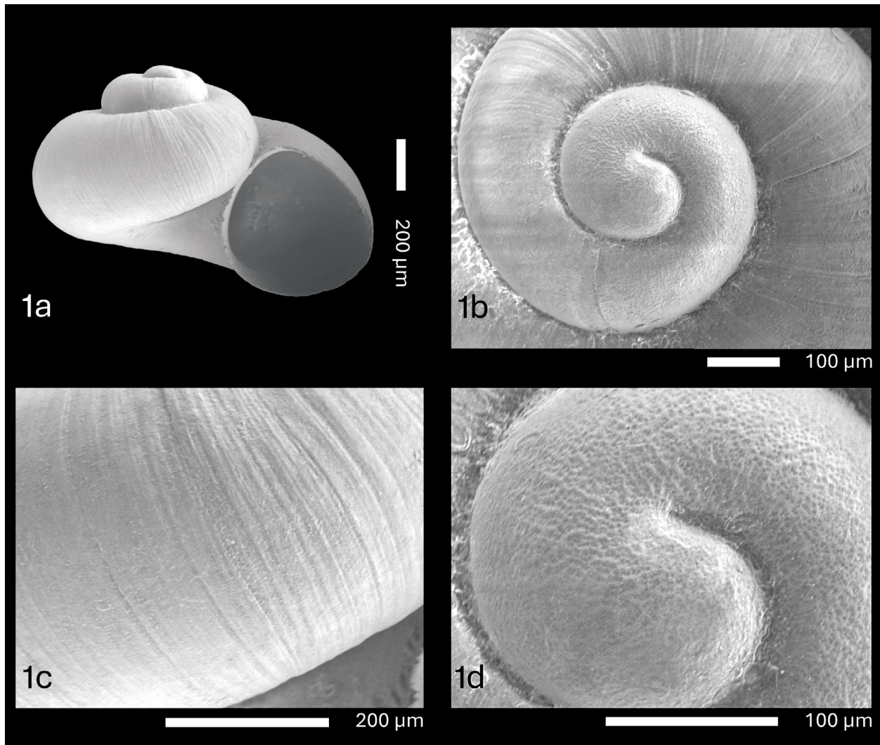
Fig. 1. SEM images of Kulyiella marginata gen. nov. spec. nov. Different views of a paratype. 1a. Frontal view. 1b. Protoconch apical view. 1c. Detail of the teleoconch. 1d. Detail of the protoconch.
