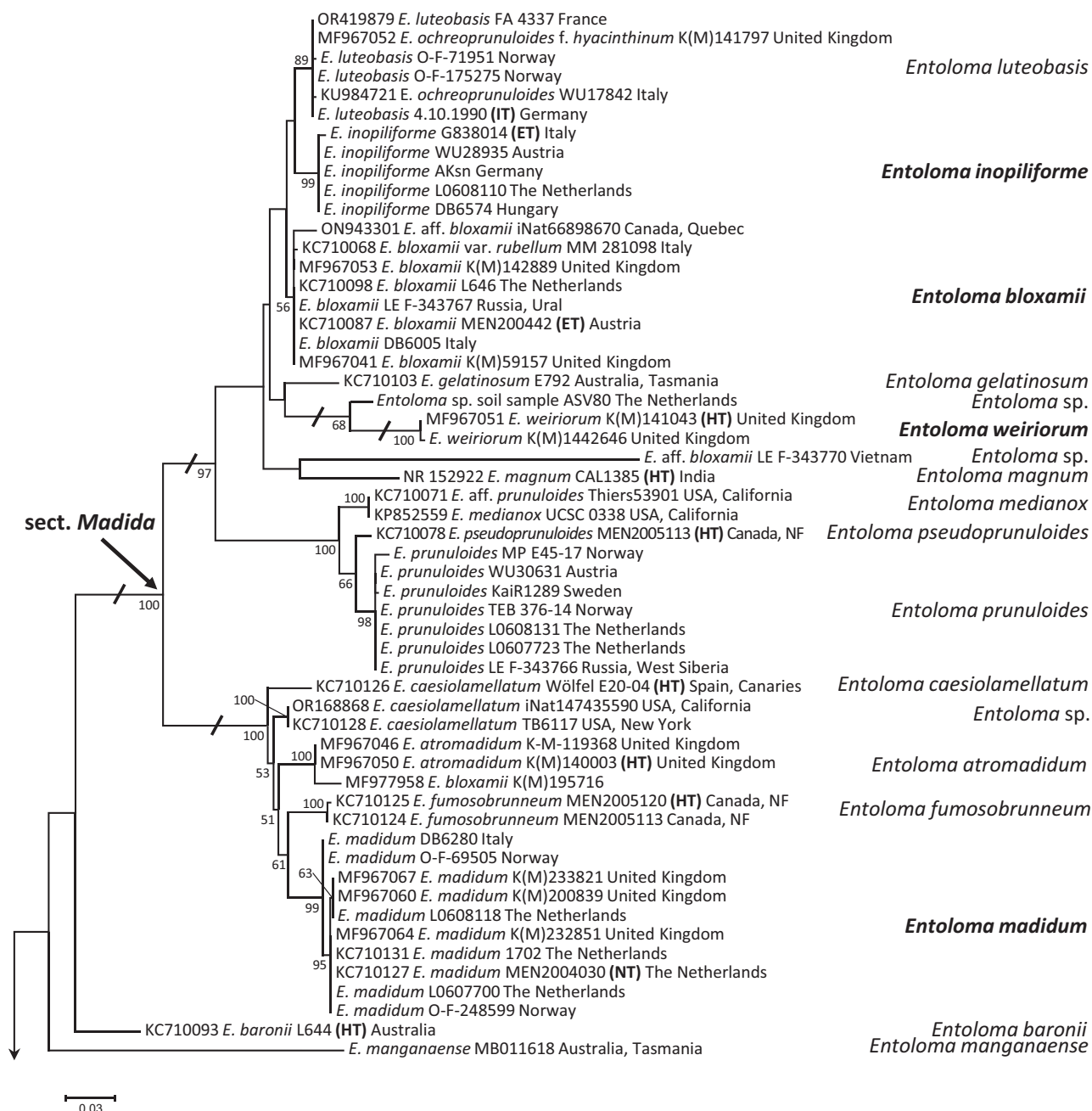
Fig. 62. Maximum Likelihood (RAxML) phylogenetic tree based on nrDNA ITS sequences of the basal grade (sect. Madida , / Turfosa , / Vinaceum , / Caeruleopolitum and / Sphagnetii ) of the genus Entoloma . ML bootstrap support values \geq 50\% are presented at the brackets. Sequences used from public databases (i.e. GenBank, UNITE) contains accession numbers, while for the newly generated sequences only voucher numbers are indicated. The country of origin is indicated in any case. Type specimens are shown as abbreviations: HT (holotype), NT (neotype), ET (epitype). The scale bar indicates expected changes per site per branch.
