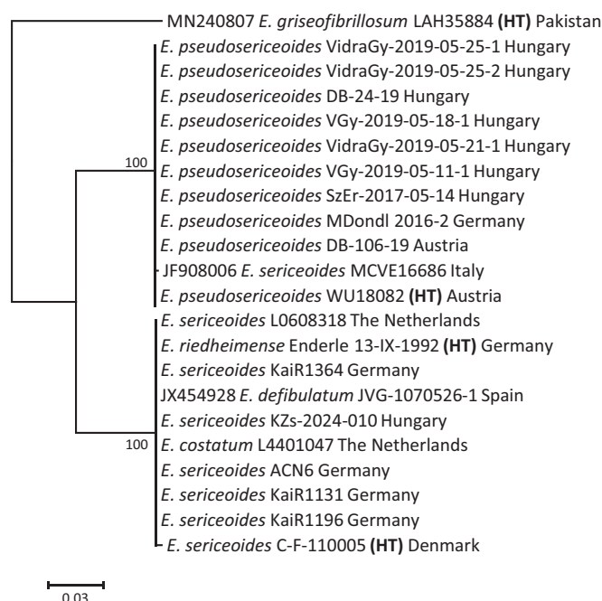
Fig. 43. Maximum Likelihood (RAxML) phylogenetic tree based on nrDNA ITS sequences depicting the relationship of Entoloma sericeoides and E. pseudosericeoides within subgen. Omphaliopsis (= Rusticoides clade) using additional sequences not included in Fig. 38. ML bootstrap support values \geq 50\% are presented at the brackets. Sequences used from public databases (i.e. GenBank, UNITE) contain accession numbers, while for the newly generated sequences only voucher numbers are indicated. Countries of origin are indicated. Type specimens are shown as abbreviations: HT (holotype), NT (neotype), ET (epitype). The scale bar indicates expected changes per site per branch.
