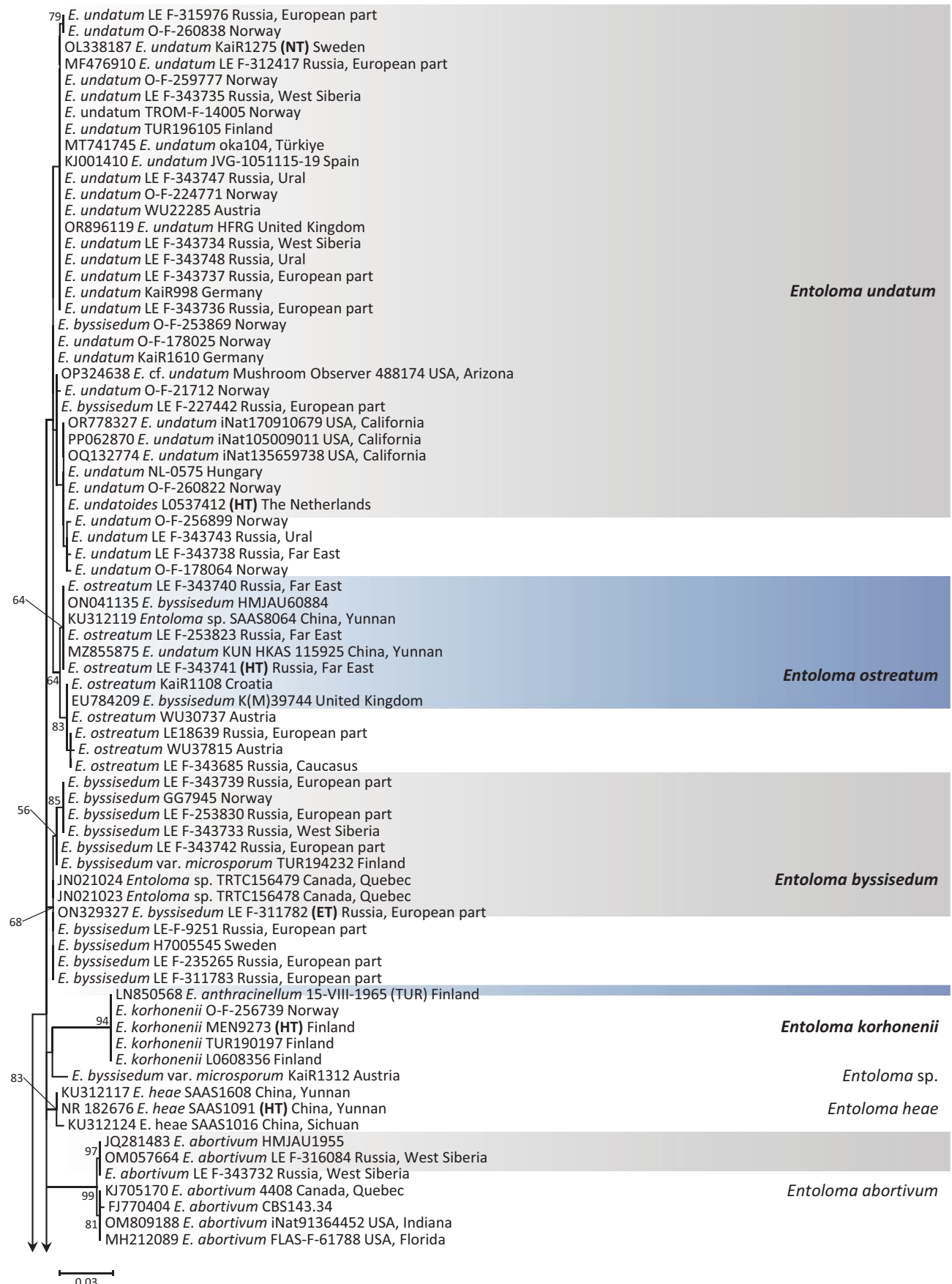
Fig. 48. Maximum Likelihood (RAxML) phylogenetic tree based on nrDNA ITS sequences of Entoloma subgen. Claudopus (= Claudopus clade). ML bootstrap support values \geq 50\% are presented at the brackets. Sequences used from public databases (i.e. GenBank, UNITE) contain accession numbers, while for the newly generated sequences only voucher numbers are indicated. Countries of origin are indicated in any case. Type specimens are shown as abbreviations: HT (holotype), NT (neotype), ET (epitype). The scale bar indicates expected changes per site per branch.
