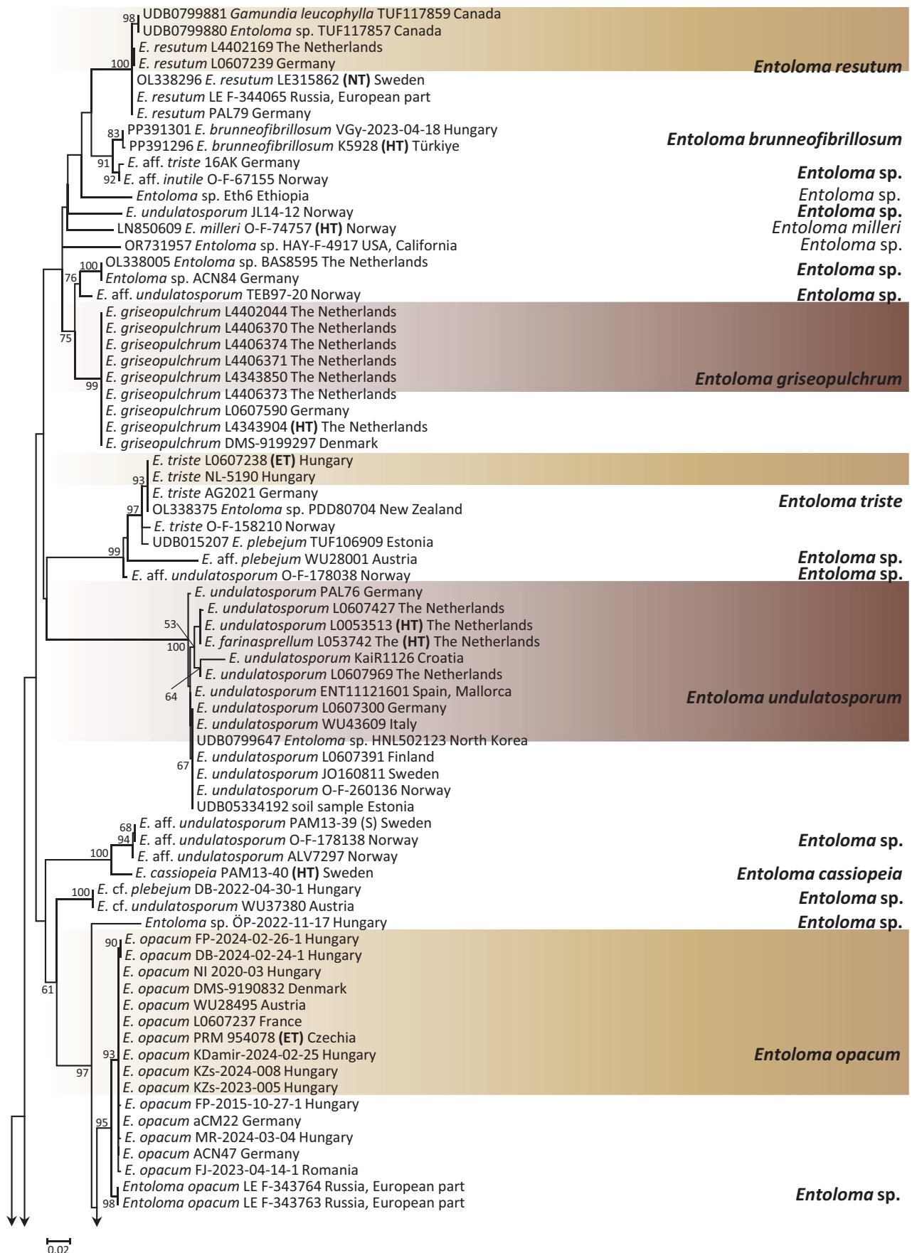
Fig. 2. Maximum Likelihood (RAxML) phylogenetic tree based on nrDNA ITS sequences of Entoloma sect. Erophila (= Undulatosporum ). ML bootstrap support values \geq 50\% are presented at the brackets. Sequences used from public databases (i.e. GenBank, UNITE) contain accession numbers, while for the newly generated sequences only voucher numbers are indicated. Countries of origin are indicated in any case. Type specimens are shown as abbreviations: HT (holotype), NT (neotype), ET (epitype). The scale bar indicates expected changes per site per branch.
