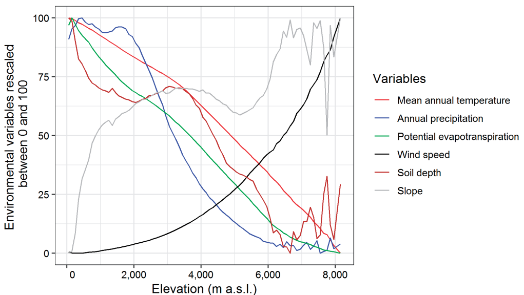
Figure 1.2. Changes in mean annual temperature, annual precipitation, potential evapotranspiration, wind speed, soil depth and slope along the Himalayan elevational gradient. Here mean values of environmental variables for 100 m elevational belts rescaled between 0-100 are plotted against elevation (for data sources, see Chapter 2).
