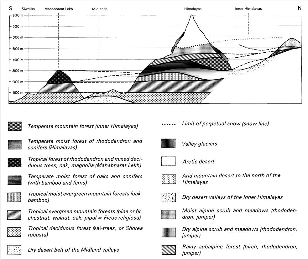
Figure 1.3. Cross-section of the vegetation of Nepal. Source: Hagen, 1998 in HMG/N/MFSC, 2002.
