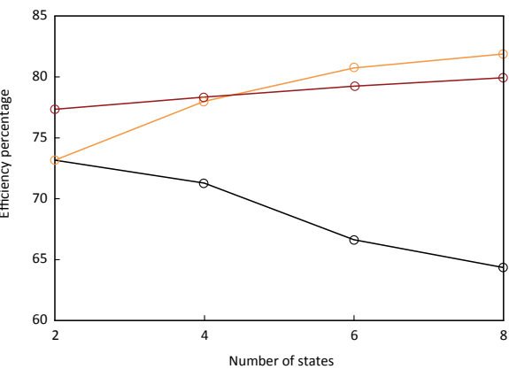
Figure 3. Impact of number of states in ordered, unordered MP, and 3ta on the efficiency of the methods. The difference in efficiency between methods was assessed by iterative recoding of the same matrices with two, four, six and eight states. Orange: ordered MP; red: 3ta; black: unordered MP.
