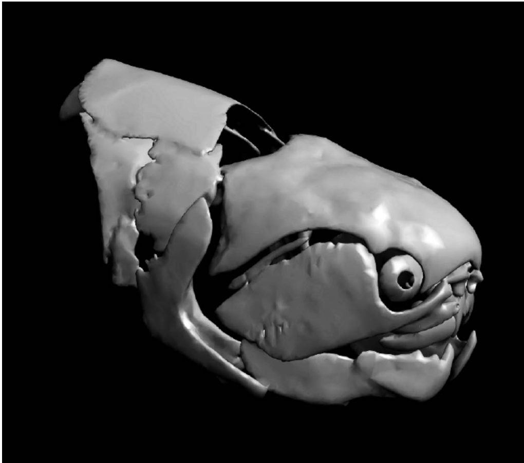
FIGURE 1—Interactive 3-D PDF of a digital surface model of the skull and dermal shoulder girdle of Dunkleosteus terrelli . Three-dimensional content can be activated by clicking on the figure (Adobe Acrobat Reader version 7 or higher required). (File is also provided as online supplemental material, see Accessibility of Supplemental Material.)
