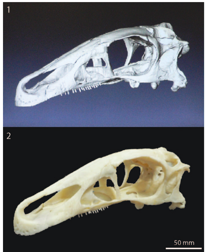
FIGURE 3—1, digital model of the reconstructed skull of Erlikosaurus andrewsi ; 2, rapid prototype based on digital model.
