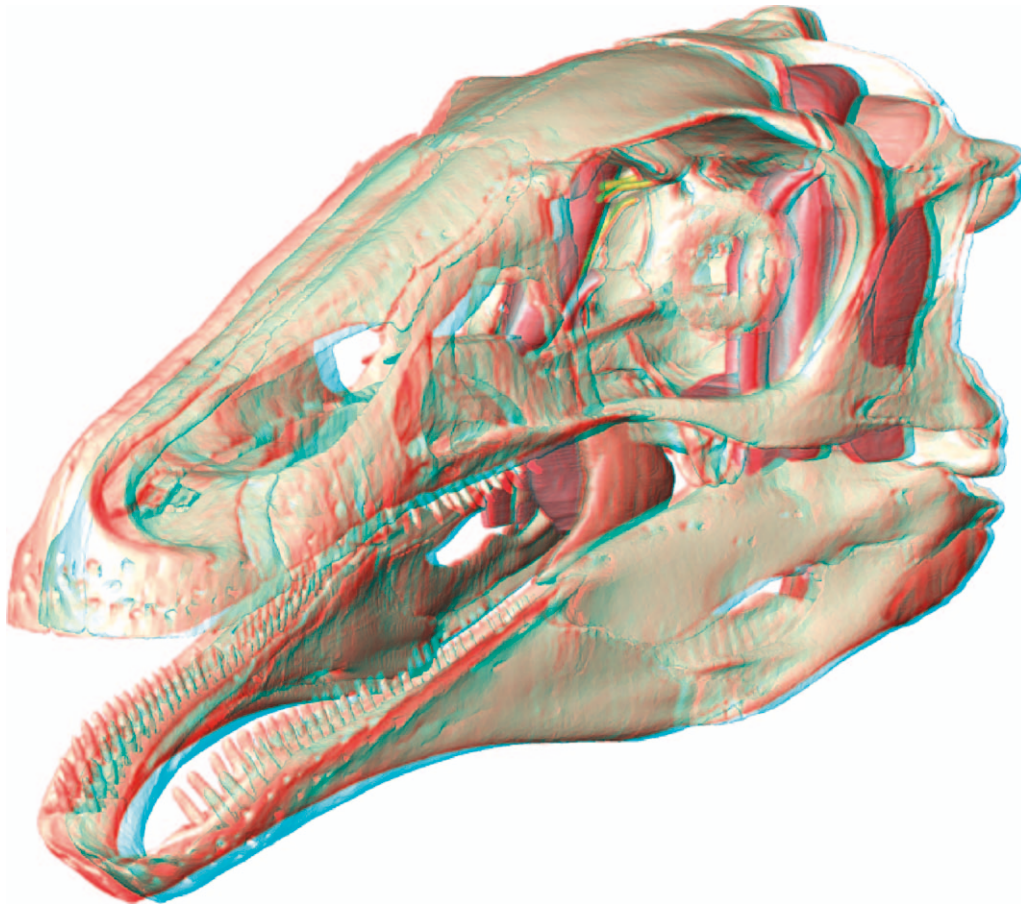
FIGURE 4—Anaglyph stereo images of Erlikosaurus andrewsi depicting the three-dimensional adductor muscle anatomy. The 3-D effect of the anaglyph image will be visible with red/blue glasses.
