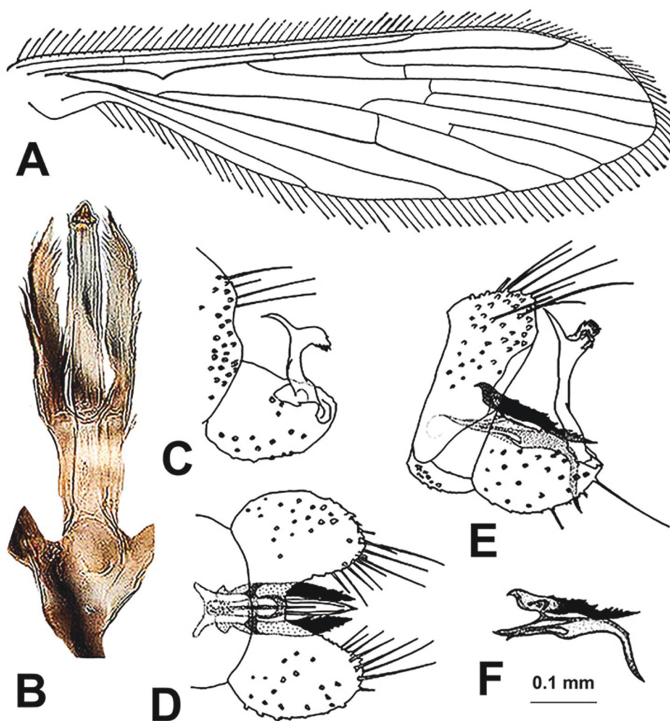
Figure 7. Tasiocera jenkinsoni . A, wing; B, aedeagal complex, dorsal view; C, hypopygium, dorsal view; D, hypopygium, ventral view; E, hypopygium, lateral view; F, aedeagal complex, lateral view. Photo of B by J. Kramer (2017). Drawing of A by Savchenko (1982), drawings of C–F by Caspers and Noll (1981). Photograph and drawings downloaded from the CCW.
