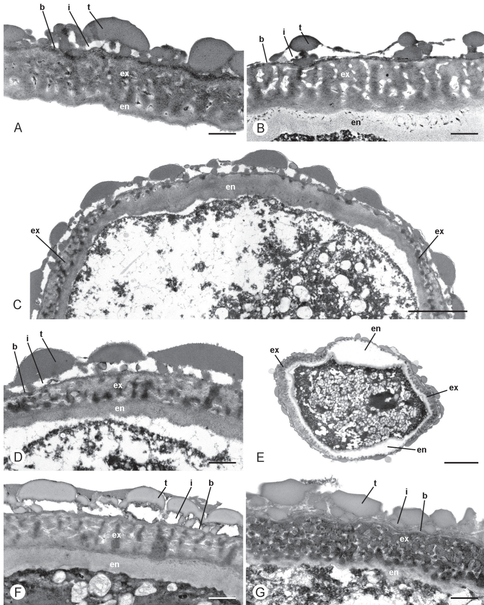
FIGURE 4. Pollen of Miliusa , TEM. A. Miliusa balansae : Detail of pollen wall with coarsely granular infratectum, tubular exintine and homogeneous endintine. B. Miliusa cuneata : Detail of pollen wall with coarsely granular infratectum, tubular exintine and homogeneous endintine. C, D. Miliusa horsfieldii (Mols 12): (C) Detail of pollen wall with coarsely granular infratectum, tubular exintine (left and right) and germination zone (middle) consisting of homogeneous endintine; (D) Detail of pollen wall with coarsely granular infratectum, tubular exintine and homogeneous endintine. E. Miliusa horsfieldii (How 71794): Pollen wall with tubular exintine (left and right) and two germination zones (top and bottom) consisting of homogeneous endintine. F. Miliusa mollis : Detail of pollen wall with coarsely granular infratectum, tubular exintine and homogeneous endintine. G. Miliusa thorelii : Detail of pollen wall with coarsely granular infratectum and tubular exintine. Scale bars – 1 µm (A, B, D, F, G), 5 µm (C), 10 µm (E); b=basal layer, en=endintine, ex=exintine, i=infratectum, t=tectum.
