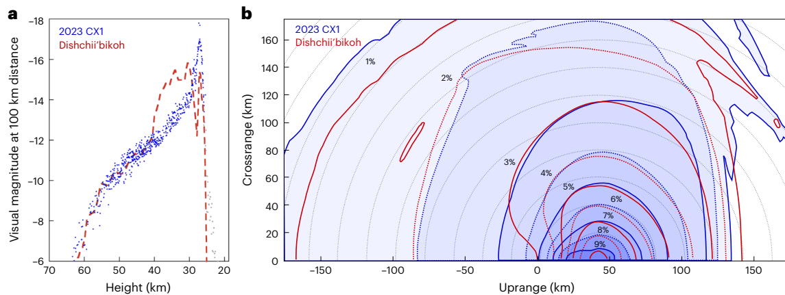
Fig. 3 | Energy deposition and ground-level overpressure for 2023 CX1 and Dishchii'bikoh. a , Energy deposition profile (on a logarithmic scale) of 2023 CX1 compared with the more common profile of Dishchii'bikoh 29 .
