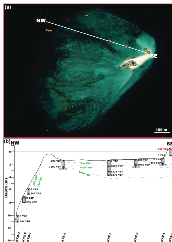
Figure 3. (a) Core transect of Kudingareng Keke on the island platform (Satellite image Bing 2024). (b) Cross section of coring transect from Kudingareng Keke. Black dates are calYBP ^{14}\text{C} dates. Red dates/* are calYBP ^{14}\text{C} dates representing an age reversal. Green dates/dashed lines are geomorphological isochrons. Core names are at the bottom. Note. Please refer to the online version of the article to view this figure in color.
