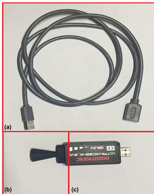
Figure 2. Ultramic384K_EVO. (a) USB cable, (b) and magnetic cone and (c) Ultramic384K_EVO device.
