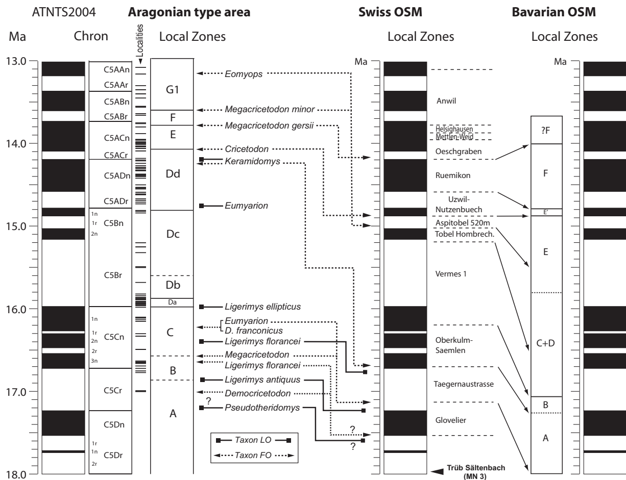
Fig. 1. Proposed correlations of the three compared European records to the ATNTS2004 (Lourens et al., 2004): Aragonian type area in North Central Spain (Daams et al., 1999a; Van Dam et al., 2006), the Upper Freshwater Molasse of the North Alpine Foreland Basin in Switzerland (Kálin and Kempf, 2009), and the Upper Freshwater Molasse in Bavaria (Abdul-Aziz et al., 2009).
