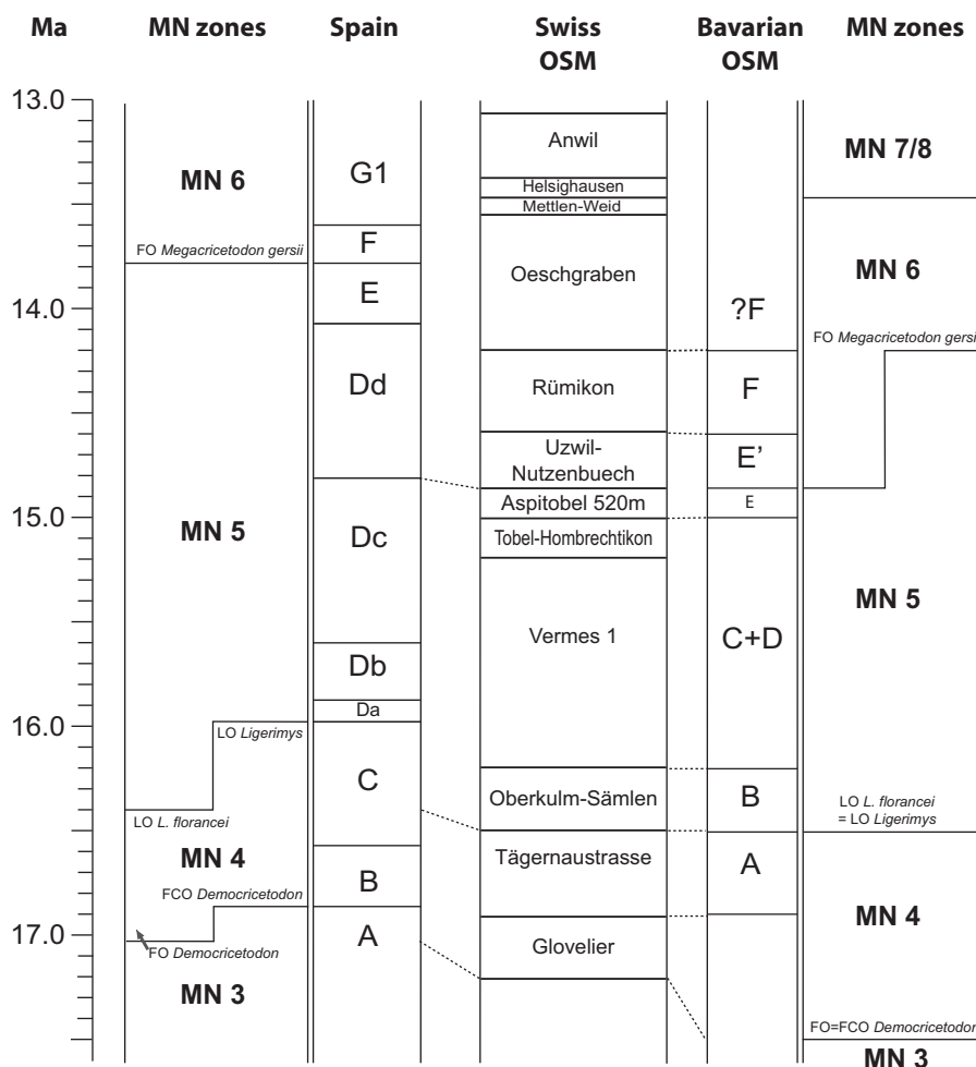
Fig. 2. Comparisons between Spanish, Swiss and German local biostratigraphies. The chronology used for the Swiss and German record is after Kälín and Kempf (2009) with the exception of the paleomagnetical correlations for the lower part of the scale which follow Schlunegger et al. (1996) (see text for discussion). Possible correlations between local biostratigraphies are indicated by dashed lines. For the distribution of the MN units, several possibilities are included, depending on the used criteria.
