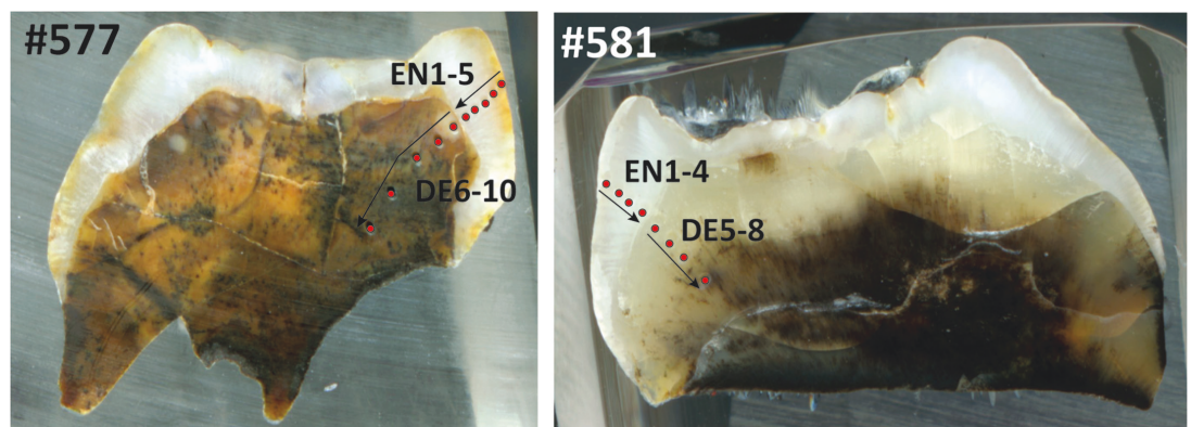
Appendix 1—figure 4. Laser ablation profiles across the two teeth from Sibrambang Cave. #577 (left) refers to specimen 11565.162; #581 (right) refers to specimen 11564.5. The red dots represent the position of the rasters, and arrows indicate the sequence of the analyses. EN = enamel. DE = dentine.
