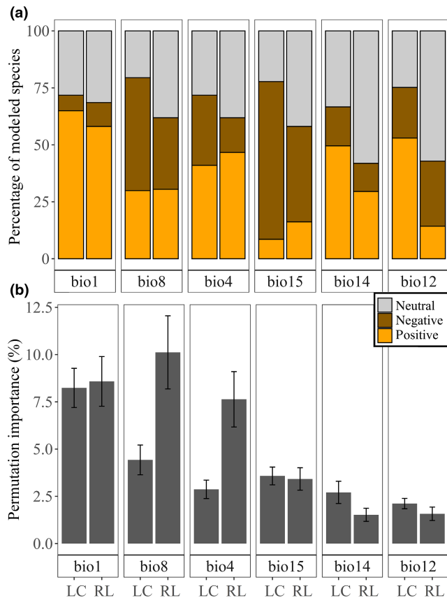
FIGURE 6 The response to annual mean temperature (bio 1), temperature seasonality (bio 4), mean daily mean air temperatures of the wettest quarter (bio 8), annual precipitation amount (bio 12), precipitation amount of the driest month (bio 14) and precipitation seasonality (bio 15) in the species distribution models of Least Concern and Red List Dutch wild bees (a) and the permutation importance with the standard error (b). The bars represent the percentage of species that showed a negative correlation (dark orange), or a positive correlation (light orange) or no significant correlation (neutral) with the bioclimatic variable.
