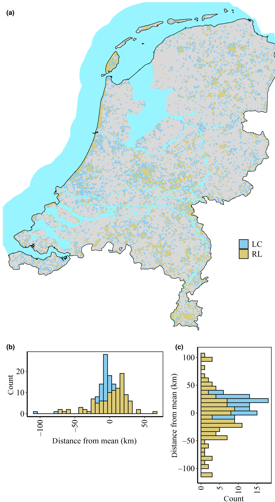
FIGURE 2 The spatial distribution of observation data for Red List and Least Concern wild bee species in the Netherlands (a) and their difference in spatial distribution on the longitudinal (b) and latitudinal (c) axis. (b, c) The distance in kilometers between the average longitude and latitude orientation of the modeled species and the average longitude and latitude values of all observations.
