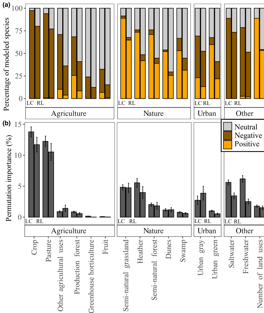
FIGURE 5 The response to different land use variables in the species distribution models of Least Concern and Red List wild bees (a) and the permutation importance with the standard error (b). The bars represent the percentage of species that showed a negative correlation (dark orange), a positive correlation (light orange), or no significant correlation (neutral) with the land use variable. For every land use category, the left stacked bars represent the Least Concern species, and the right stacked bars represent the Red List species.
