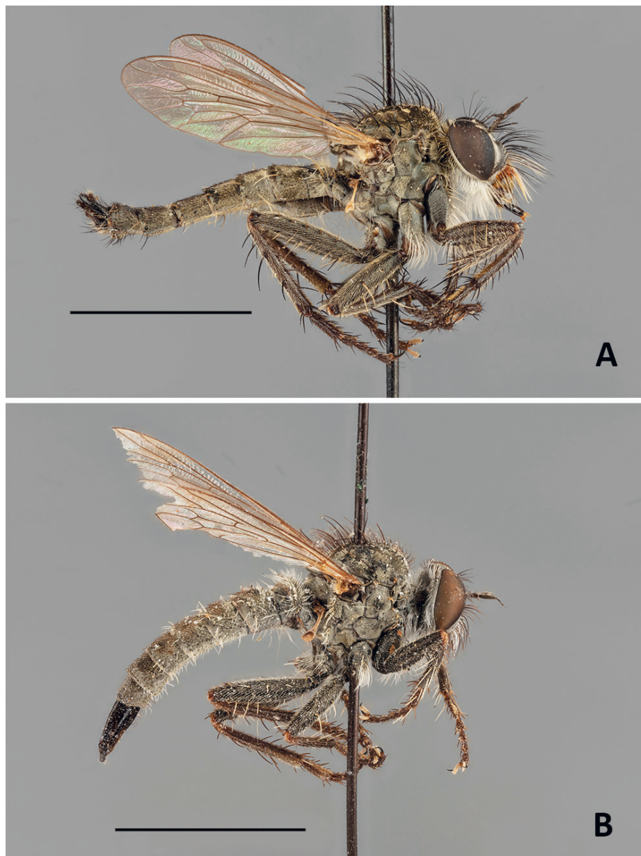
Figure 7. A holotype of Conosiphon pauper (Becker, 1907), male habitus in lateral view B syntype of Conosiphon similis Becker, 1923, female habitus in lateral view. Scale bars: 5 mm. Photographs: E. Wolff, courtesy of J. Pohl, ZMHB.
