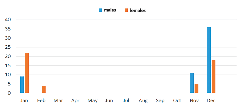
Figure 10. Graphic showing the flight period of Conosiphon ianus Álvarez Fidalgo & van den Broek, sp. nov., based on the 105 records gathered from collections and photographs. Graph: M. Álvarez Fidalgo.
