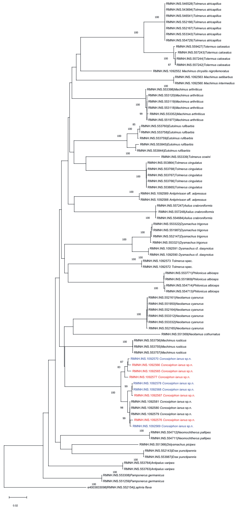
Figure 11. Neighbour-Joining tree for Conosiphon ianus Álvarez Fidalgo & van den Broek, sp. nov., and related genera of the subfamily Asilinae. Laphria flava (Linnaeus, 1761) is used as an outgroup. Red indicates dark-winged males and blue indicates clear-winged males of C. ianus .
