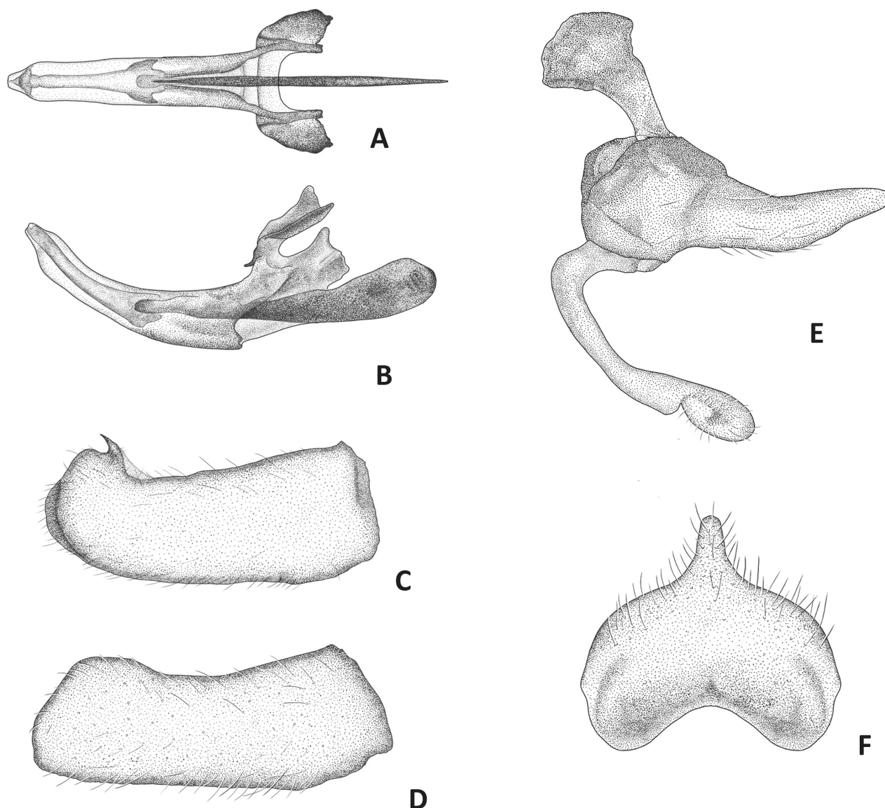
Figure 3. Conosiphon ianus Álvarez Fidalgo & van den Broek, sp. nov., male terminalia A phallus in dorsal view B phallus in lateral view C right epandrium in dorsal view D right epandrium in lateral view E left gonocoxite and gonostylus in lateral view F hypandrium. Drawings: M. Trillo Camprodón.
