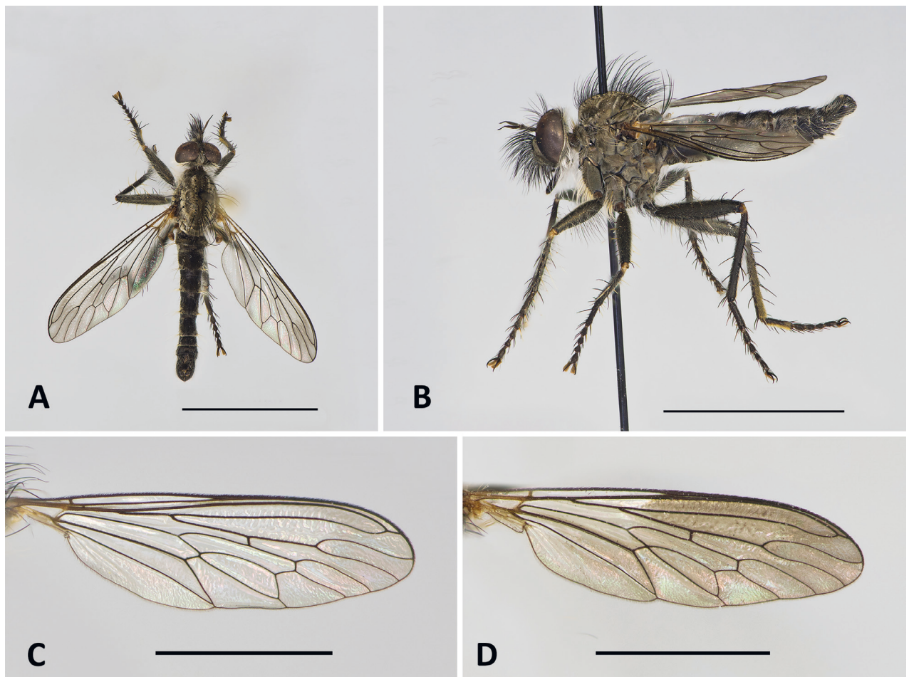
Figure 2. Conosiphon ianus Álvarez Fidalgo & van den Broek, sp. nov., male holotype (MNCN_Ent 344922) A habitus in dorsal view B habitus in lateral view Male paratype of the clear-winged form (PAFC) C wing. Male paratype of the dark-winged form (PAFC) D wing. Scale bars: 5 mm ( A , B ); 3 mm ( C , D ). Photographs: PÁF.
