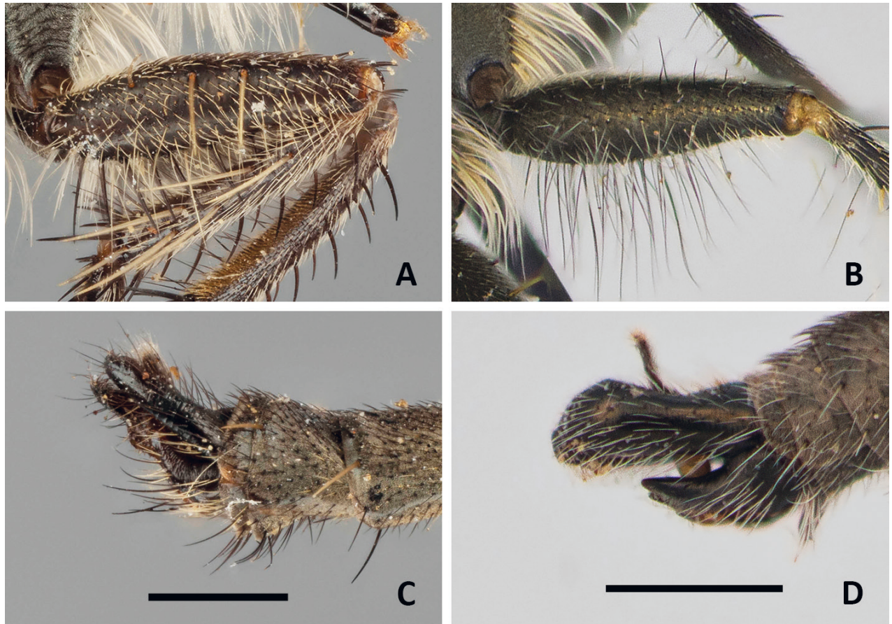
Figure 12. Holotype (male) of Conosiphon pauper (Becker, 1907) A fore femora, showing macrosetae present on ventral side C terminalia in lateral view. Photos: E. Wolff, courtesy of J. Pohl, ZMHB. Paratype (male) of Conosiphon ianus Álvarez Fidalgo & van den Broek, sp. nov. B fore femora, showing filiform setae present on ventral side D terminalia in lateral view. Scale bars: 1 mm. Photographs: PÁF.
