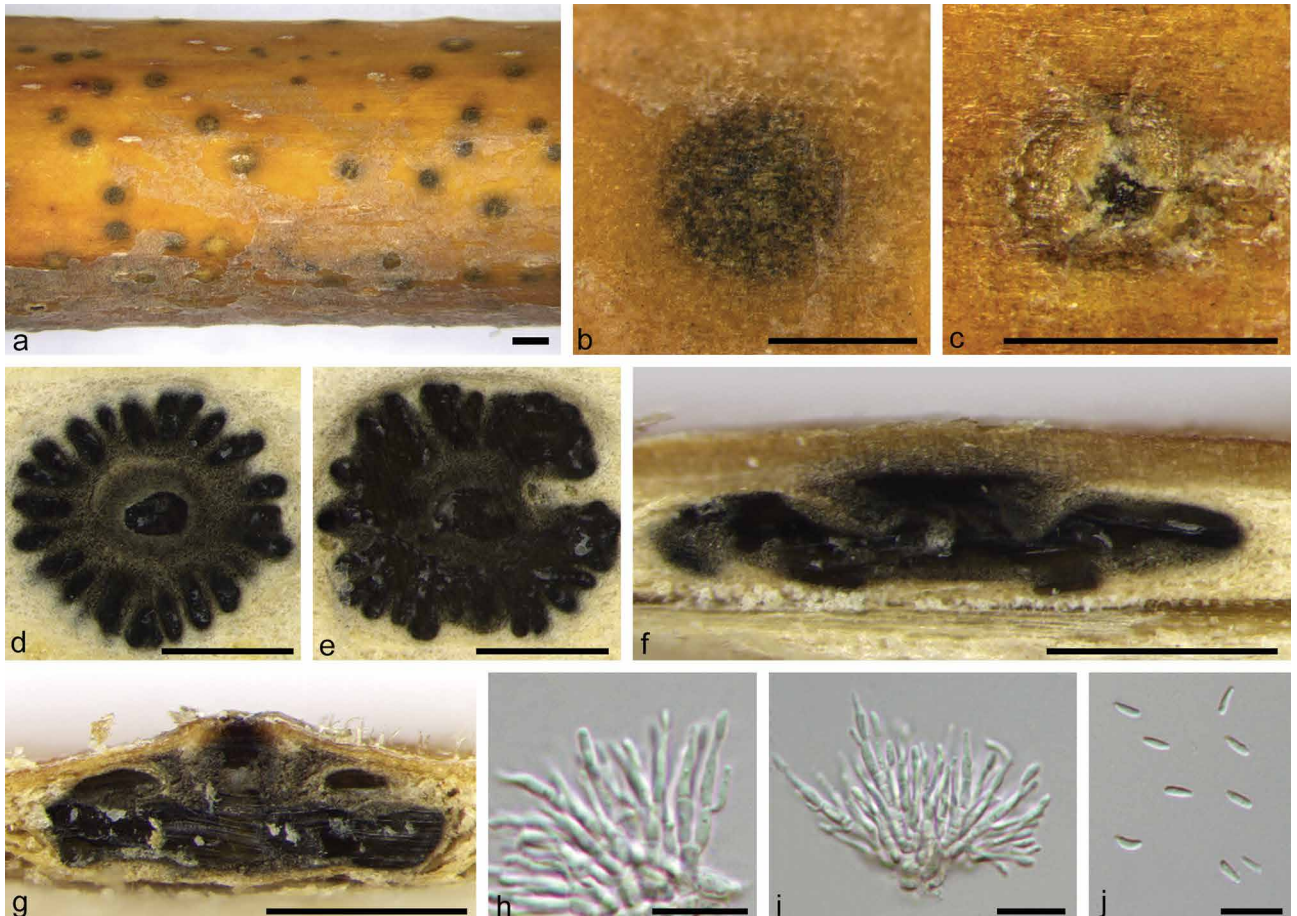
Fig. 5 Cytospora ailanthicola on Ailanthus altissima (BJFC-S550). a–c. Habit of conidiomata on branch; d–e. transverse section through conidiomata; f–g. longitudinal section through conidiomata; h–i. conidiogenous cells with attached conidia; j. conidia. — Scale bars: a = 1 mm; b–g = 0.5 mm; h–j = 10 µm.
