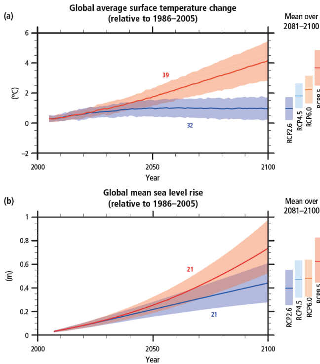
FIG. 1.1: Modelled changes in global average surface temperature (a) and global mean sea level rise (b) from 2006 to 2100. The lowest and highest emission scenarios are shown. Coloured bars at the right hand side show the mean and uncertainty for all scenarios. The number above the lines refers to the number of models used to calculate the multi-model mean. Source: figure taken from IPCC (2014).
