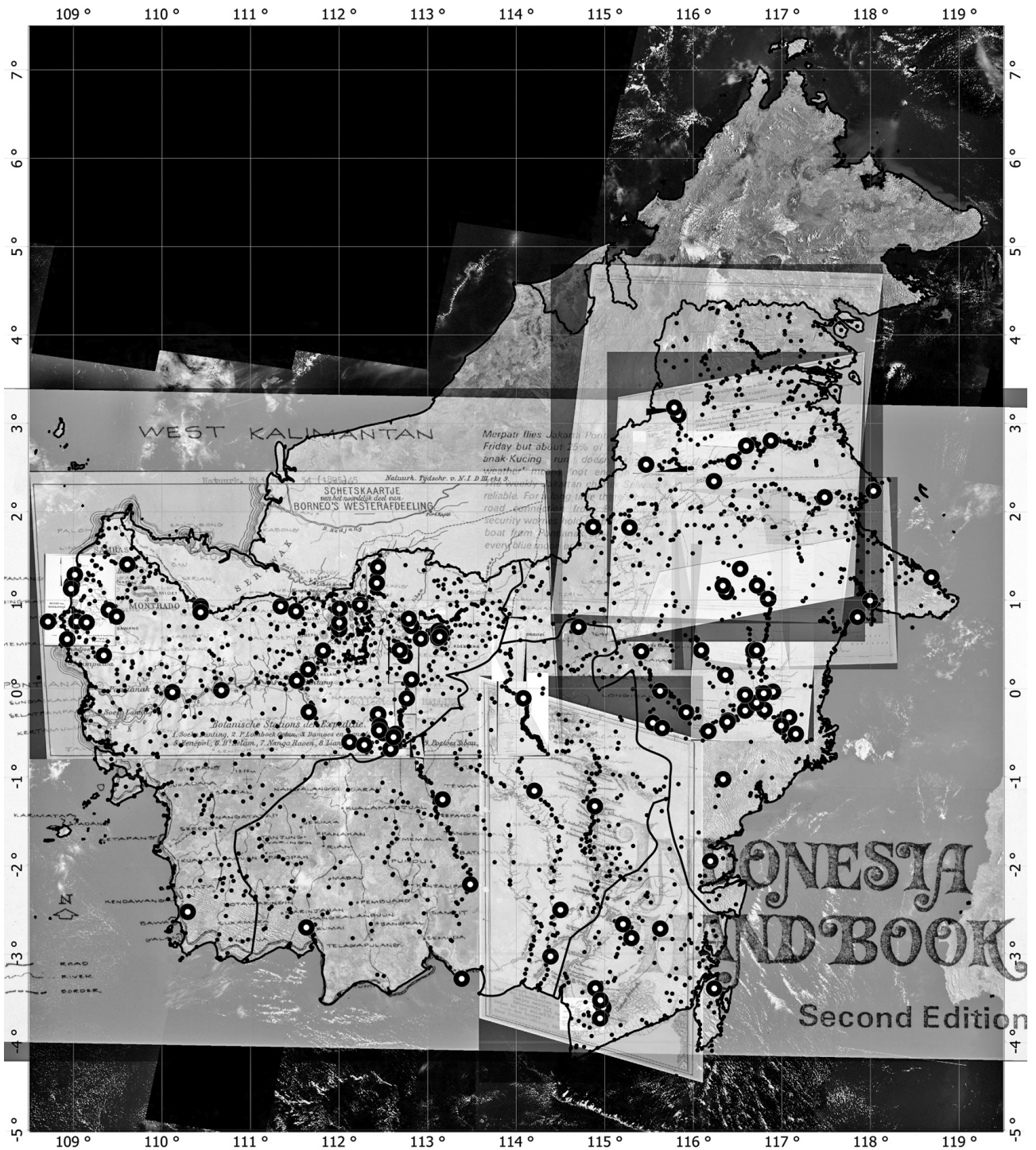
Fig. 1 Landsat 7 image of Borneo (geographic projection) superimposed with a selection of georegistered digitized maps. Black dots indicate georeferenced localities retrieved from the maps. White dots indicate georeferenced localities where actual collections were made which otherwise could not have been georeferenced.
