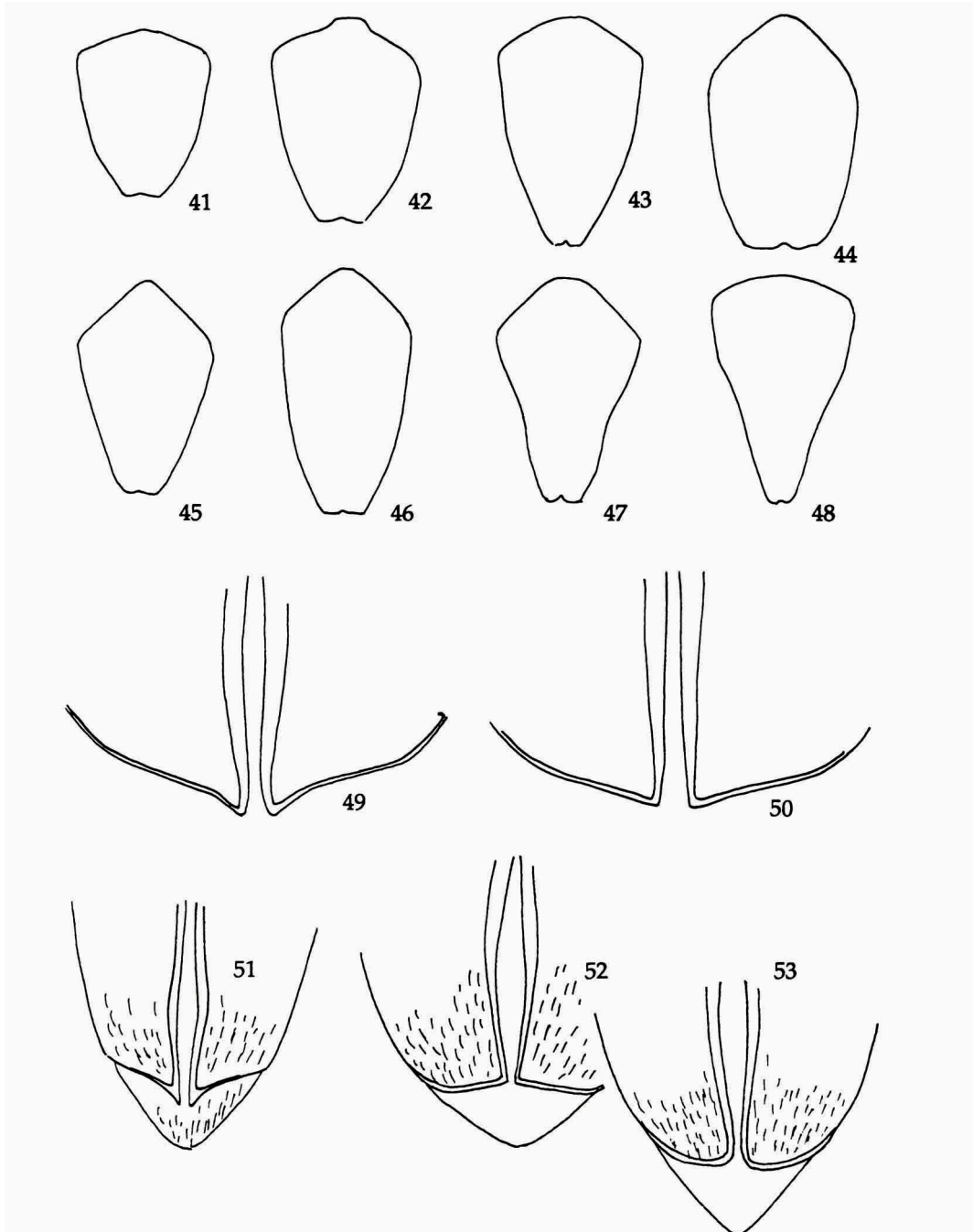
Figs. 41-53; 41, Choleva agilis (Illiger, 1798), ♀, France, Lille (ITZ); 42, 46, id., ♀, Denmark, Herlev (ZMK); 43, id., ♀, Netherlands, Haamstede (NNM); 44, id., ♀, Great Britain, Cowley (BMNH); 45, id., ♀, France, St. Germain (ITZ); 47, id., ♀, Great Britain, New Forest (BMNH); 48, id., ♀, Netherlands, Brummen (NNM); 49, 50, C. septentrionis septentrionis Jeannel, 1923, ♀, Sweden, Ragunda (UZMH); 51, C. septentrionis holsatica Benick & Ihssen, 1937, ♀, BRD, Bad Segeberg (author's collection); 52, C. septentrionis gracilentata Szymczakowski, 1957, ♀, Poland, Pod Sokola Góra (UZMH). 53, id., ♂, Poland, Studnisko (BMNH). 41-48, genital tergite, dorsal aspect; 49-53, elytral apices, dorso-caudal aspect.
