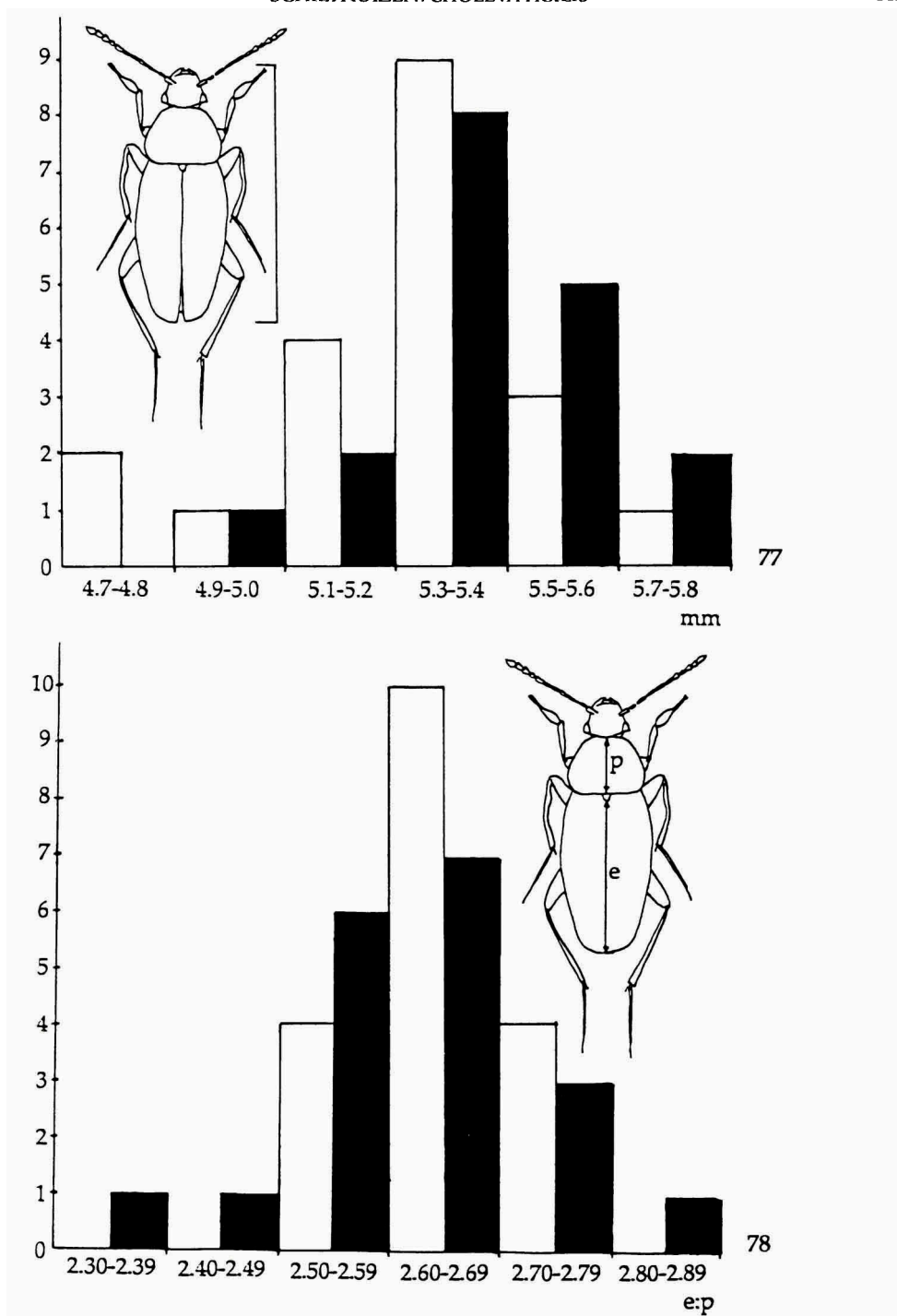
Figs. 77-78, Choleva lederiana Reitter, 1901, Finland, Lohja, Torhola Cave (UZMH). 77, distribution of bodylength among the studied specimens; black bars represent \sigma\sigma , white bars represent \text{♀♀} ; 78, distribution of values of elytral length:pronotal length among the studied specimens; black bars represent \sigma\sigma , white bars represent \text{♀♀} .
