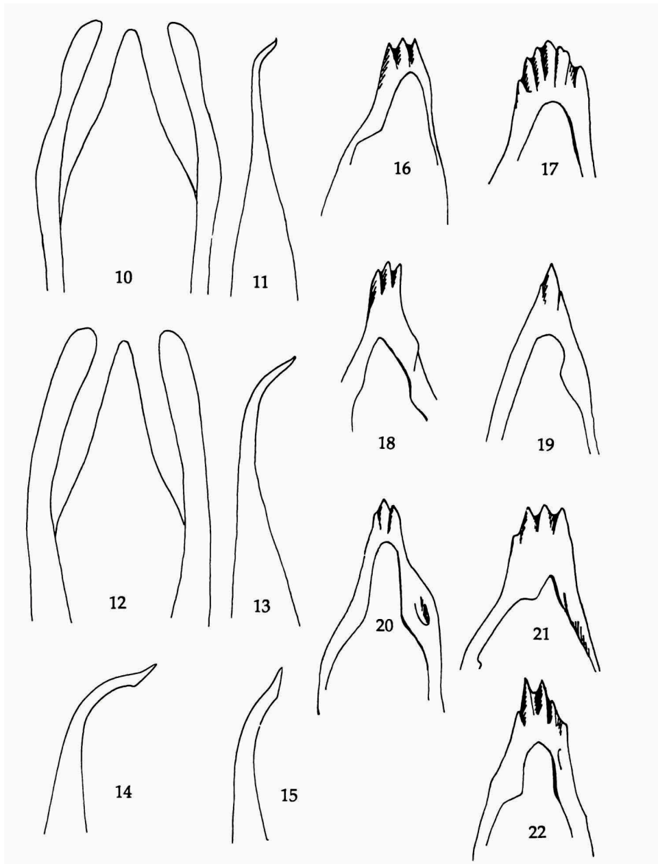
Figs. 10-22; 10,11, Choleva septentrionis holsatica Benick & Ihssen, 1937, ♂, BRD, Segeberg (author's collection); 12,13, C. septentrionis gracilentata Szymczakowski, 1957, ♂, Poland, Pod Sokola Góra (UZMH); 14, 19, C. lederiana Reitter, 1901, ♂, Finland, Lohja (UZMH); 15, C. agilis (Illiger, 1798), ♂, Netherlands, Velsen (ITZ); 16, C. septentrionis septentrionis Jeannel, 1923, ♂, Norway, Haus (ZMBG); 17, id., ♂, Great Britain, Harlech (BMNH); 18, C. lederiana Reitter, 1901, ♂, U.S.S.R., Varniechny (ZIL); 20, id., ♂, Norway, Nordkapp (ZMB); 21, C. agilis (Illiger, 1798), ♂, France, Vélizy (BMNH). 22, id., ♂, Netherlands, Schiedam (author's collection). 10, 12, aedeagal apex, dorsal aspect; 11, 13-15, aedeagal apex, lateral aspect; 16-22, ventral tooth of the internal sack, dorsal aspect.
