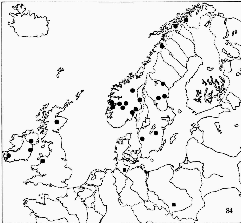
Figs. 83-84. 83, stippled areas indicate possible areas of contact between two species; 84, geographical distribution of Choleva septentrionis Jeannel, 1923; squares indicate the localities of the two cavernicolous subspecies: C. septentrionis holsatica Benick & Ihssen, 1937 in Germany and C. septentrionis gracilentia Szymczakowski, 1957 in Poland.
