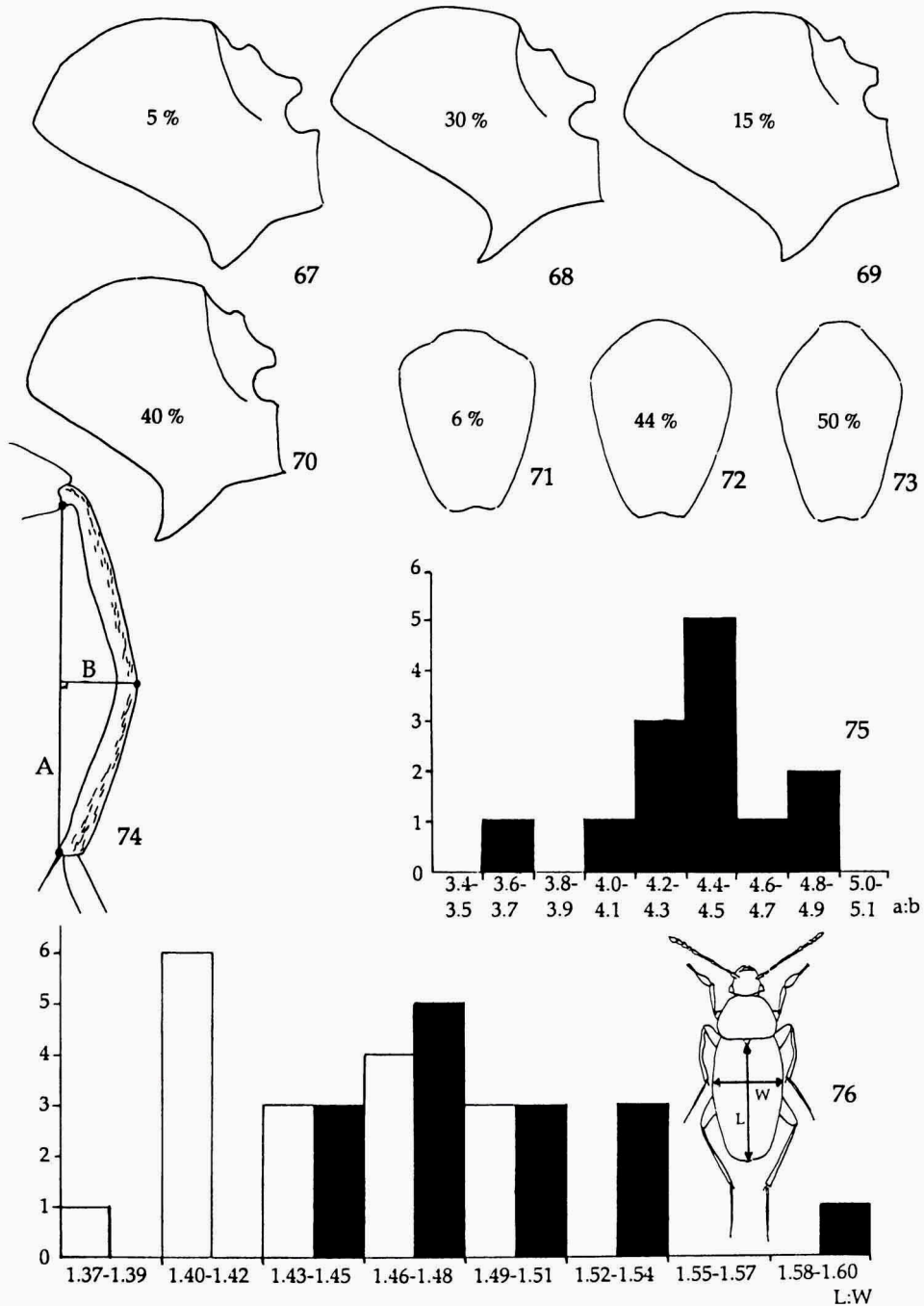
Figs. 67-76, Choleva lederiana Reitter, 1901, Finland, Lohja, Torhola Cave (UZMH). 67-70, ♂♂, meta-ochanther, dorsal aspect; percentages indicating the proportion of the studied specimens that show a similar shape; 71-73, ♀♀, genital tergite, dorsal aspect; percentages indicating the proportion of the studied specimens that show a similar shape. 74, ♂, mesotibia; indicated are the positions of A and B; 75, ♂♂, distribution of values of A:B among the studied specimens; 76, distribution of elytral indices among the studied specimens; black bars represent ♂♂, white bars represent ♀♀.
