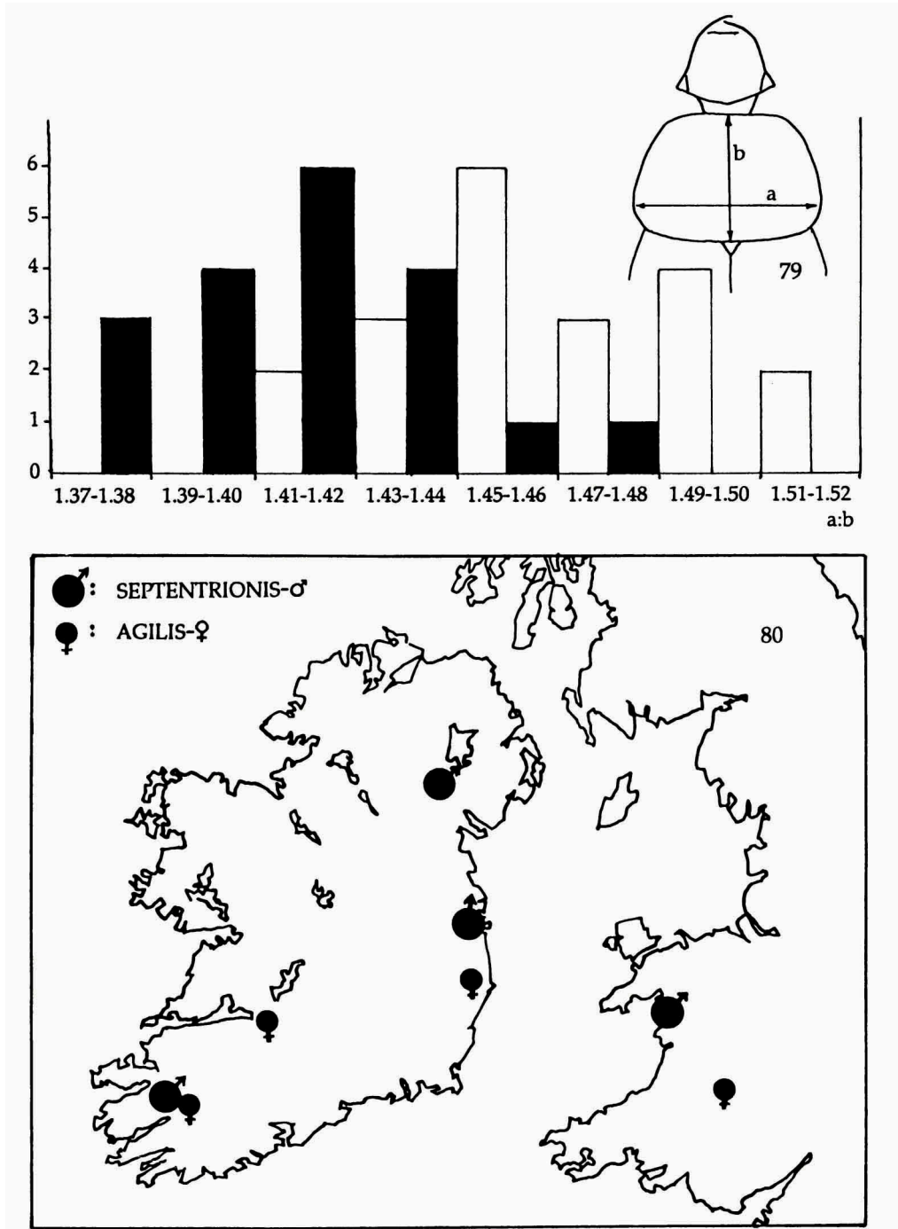
Figs. 79-80. 79, Choleva lederiana Reitter, 1901, Finland, Lohja, Torhola Cave (UZMH); distribution of pronotal indices among the studied specimens; black bars represent ♂♂, white bars represent ♀♀; 80, geographical distribution of ♂♂ C. septentrionis septentrionis Jeannel, 1923 and ♀♀ C. agilis (Illiger, 1798) in Ireland and Wales.
