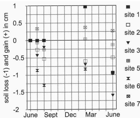
Fig. 29. Soil loss and gain from the seven erosion stake sites (site 4 omitted).
