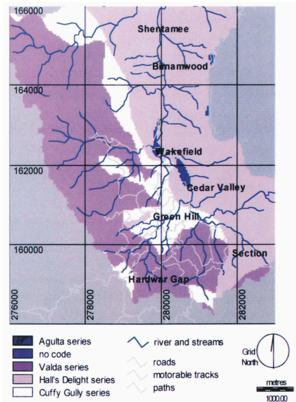
Fig. 17. An alternative qualitative soil parameter scoring system (after CIDA & Forestry and Soil Conservation Department, 1993).
