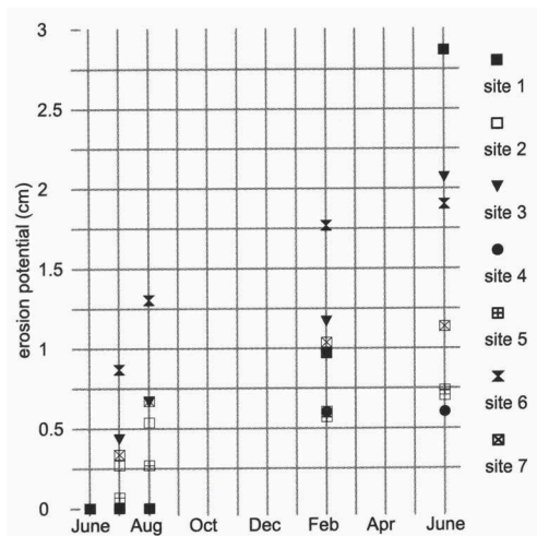
Fig. 30. Cumulative erosion potential (CEP) for six of the seven erosion stake sites.
