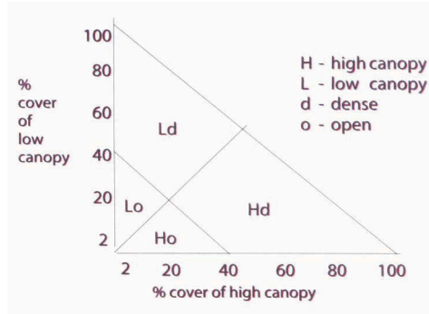
Fig. 9. Canopy height and density parameters (after Gils & Wijngaarden, 1984).
