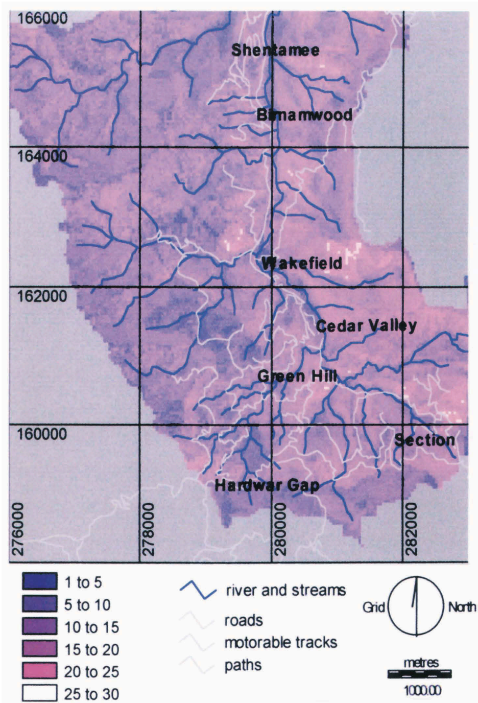
Fig. 20. E5 image using alternative qualitative soil parameters (after CIDA & Forestry and Soil Conservation Department, 1993).
