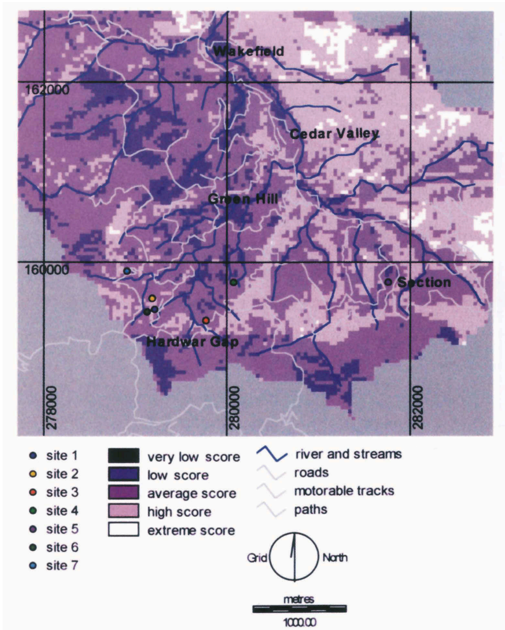
Fig. 28. Location of erosion stake sites with model result (E5) as background.
