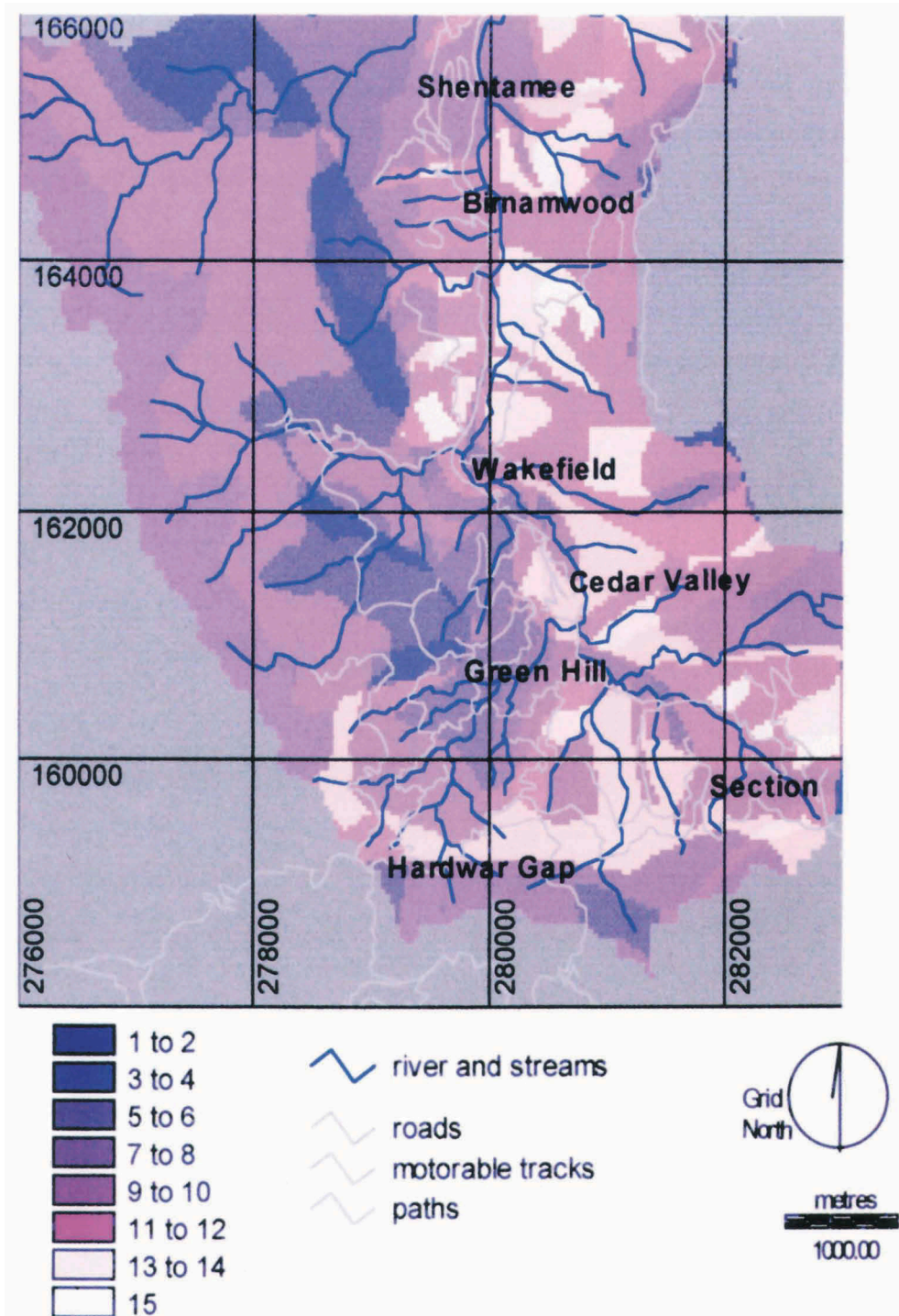
Fig. 15. Erosion scores for E4 Earth.
