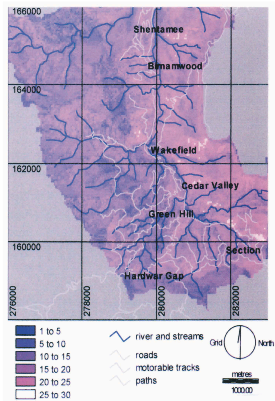
Fig. 22. E5 image using alternative vegetation parameters taking litter into account.
