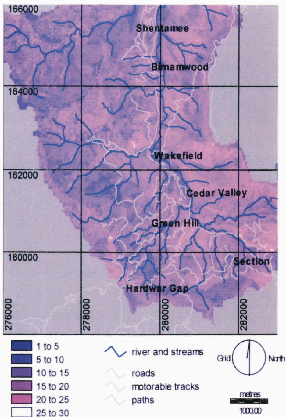
Fig. 21. E5 image using alternative USLE soil parameters (after Loch & Pocknee, 1995).
