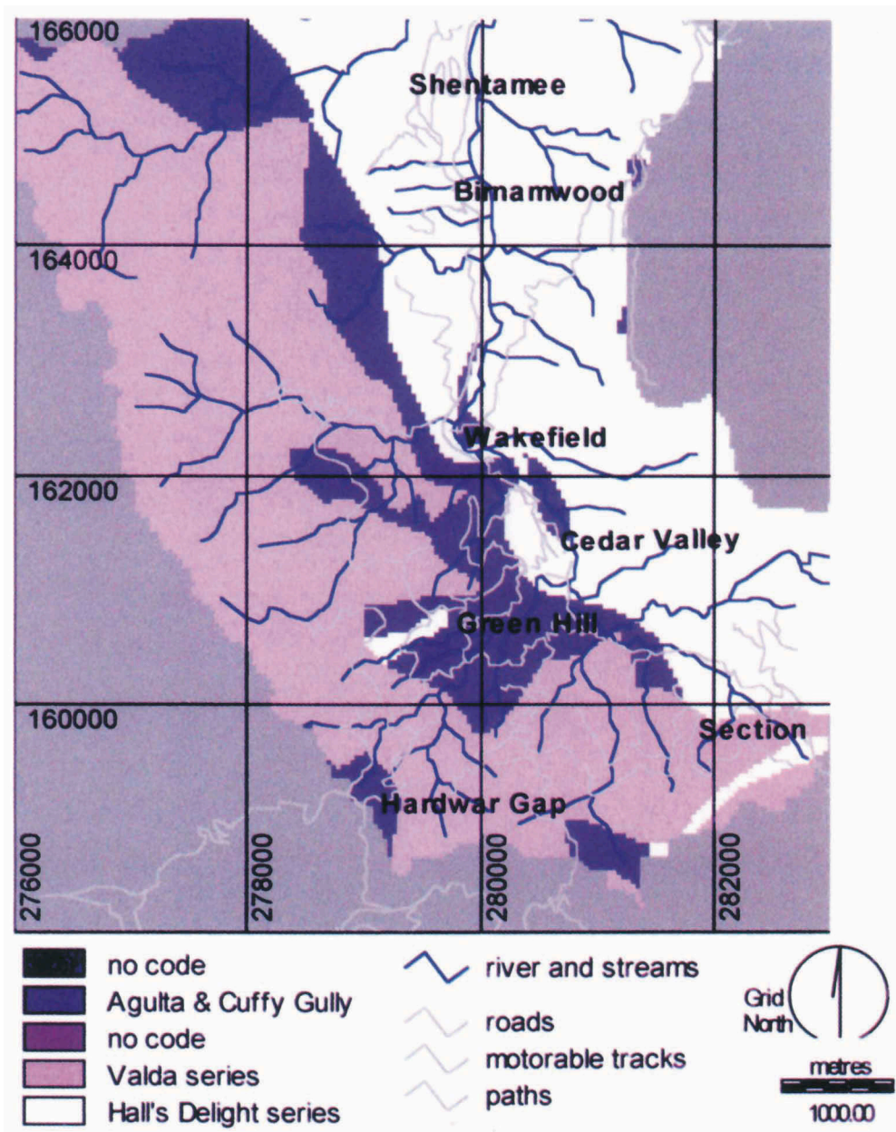
Fig. 8. Soils classes (series names: 23=Agulta; 38/305/306=Cuffy Gully; 46/301=Hall's Delight; 52=Valda).
