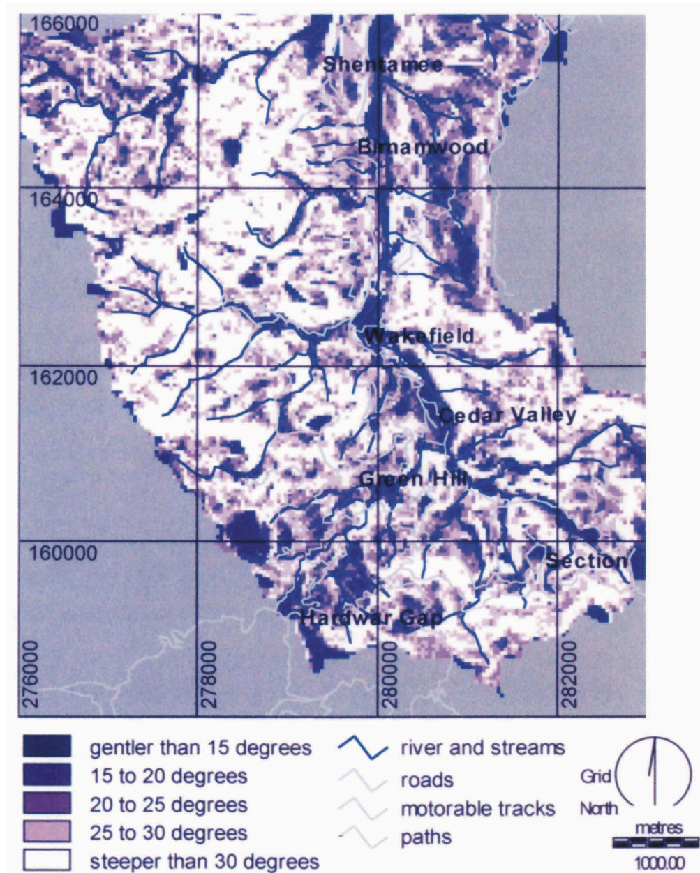
Fig. 6. Slope angle classes (in degrees).
