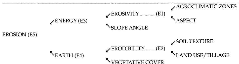
Fig. 4. The cartographic model in general detail (see Appendix 4 for file inputs).
