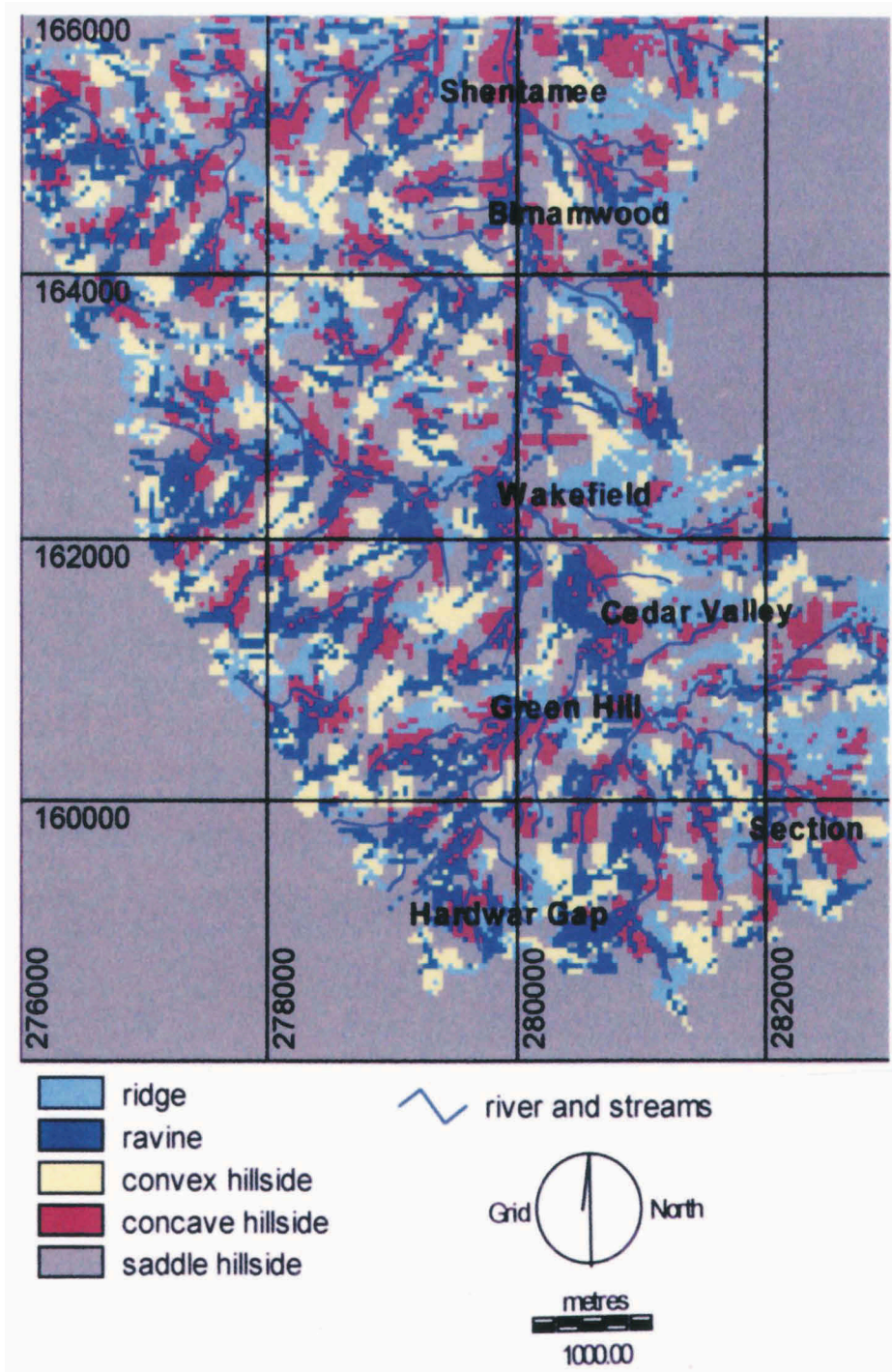
Fig. 26. Selection of topographic elements generated by the TOPOSHAPE module.
