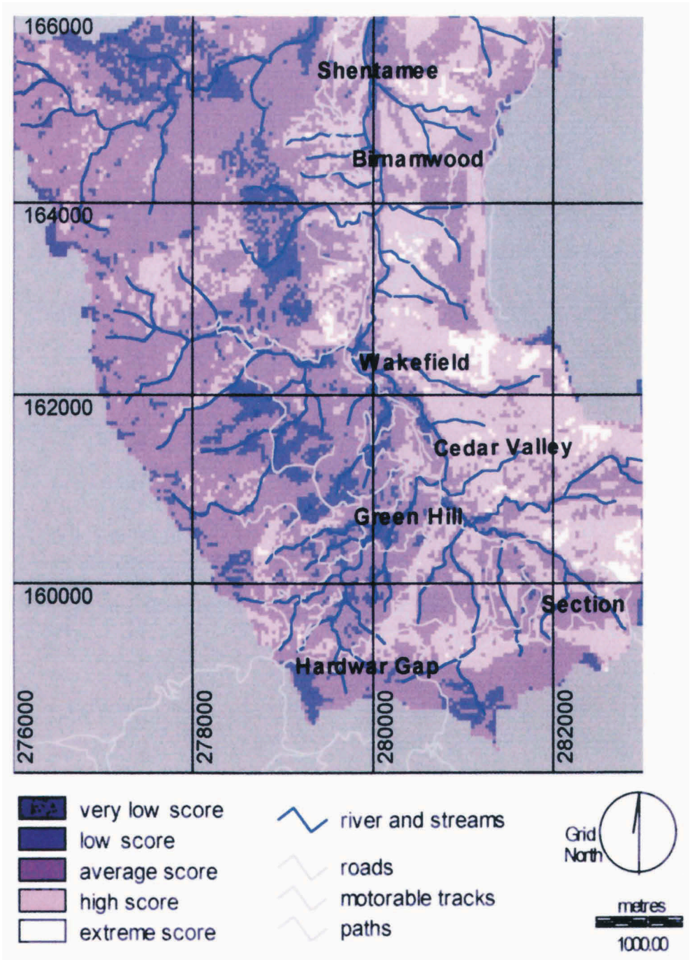
Fig. 16. Erosion classes for E5 Erosion (reclassified into 5 classes from the E5 erosion scores).
