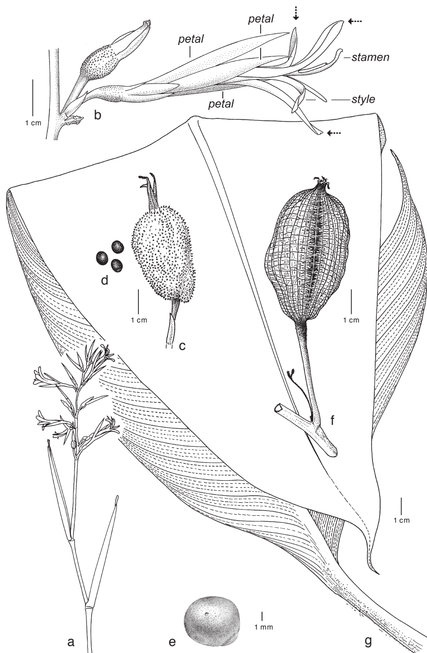
Fig. 9. Canna tuerckheimii Kraenzl. a. Inflorescence; b. detail of flower showing sepals, petals, staminodes (marked by arrows), stamen, and style; c. fruit; d. seeds; e. detail of seed showing stomata and elevated area; f. old fruit after shedding of the tubercles; g. leaf (a: Maas & Dressler 1614 , drawn from a colour slide; b: Maas & Cobb 4707 , drawn from a colour slide; c–e: Maas & Cobb 4796 ; f: Davidse 24594 ; g: Maas & Dressler 1614 ).
