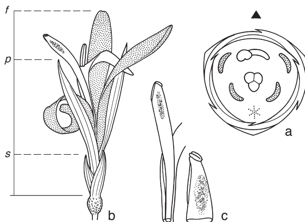
Fig. 2. Flowers of Canna (f = length of flower; p = length of petals; s = length of sepals). a. Floral diagram: androecium composed of 2 staminodes and 1 stamen in inner whorl, and 2 staminodes in outer whorl (star represents missing staminode); b. flower of C. indica showing 2 of the 3 calyx lobes, 2 of the 3 petals, 3 staminodes, 1 stamen with petaloid part and theca, and style with stigmatic areas on the top and a patch of pollen aside; c. details of style showing stigmatic areas and patch of pollen deposited on surface (a: Kress 1990, f. 1; b: Eichler 1873, t. 2, f. 1; c: Idem, t. 2, f. 3–4).
