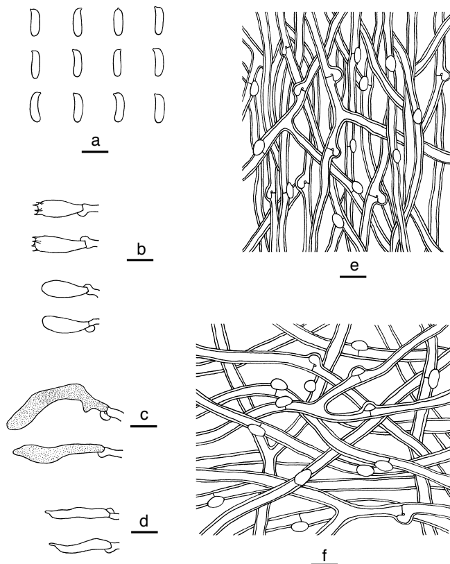
Fig. 7 Microscopic structures of Cyanosporus mongolicus . a. Basidiospores; b. basidia and basidioles; c. gloeocystidia; d. cystidioles; e. hyphae from trama; f. hyphae from context (all: holotype). — Scale bars: a = 5 µm; b–f = 10 µm.
