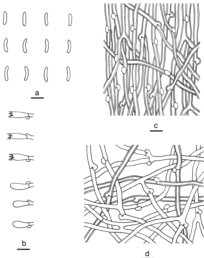
Fig. 11 Microscopic structures of Cyanosporus ungulatus . a. Basidiospores; b. basidia and basidioles; c. hyphae from trama; d. hyphae from context (all: holotype). — Scale bars: a = 5 \mu m; b–d = 10 \mu m.
