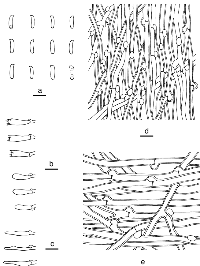
Fig. 12 Microscopic structures of Postia sublowei . a. Basidiospores; b. basidia and basidioles; c. cystidioles; d. hyphae from trama; e. hyphae from context (all: holotype). — Scale bars: a = 5 \mu m; b–e = 10 \mu m.
