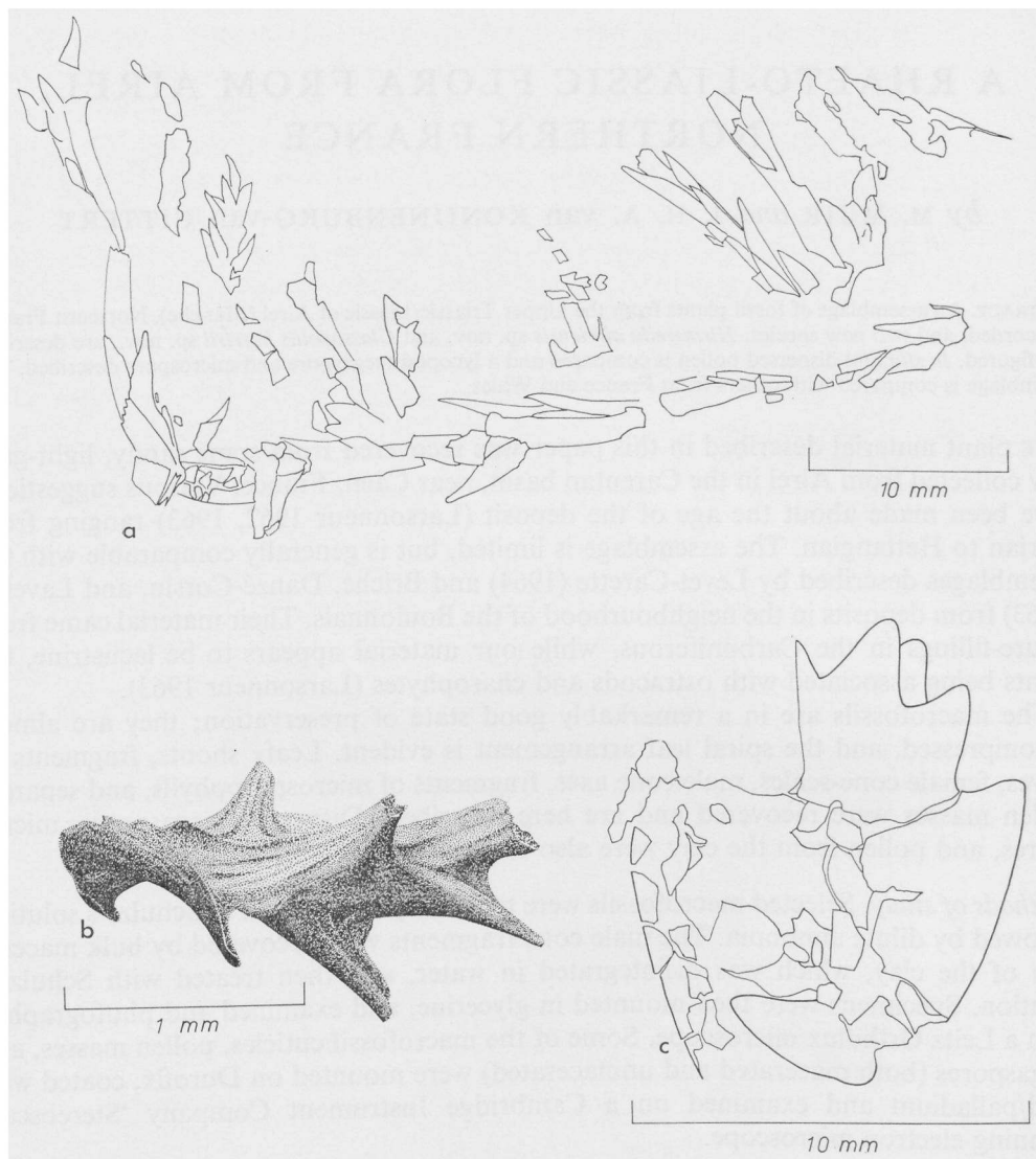
TEXT-FIG. 1. Hirmerella airelensis sp. nov. a , Holotype; \times 2.5 . b , Isolated male cone axis; \times 30 . c , Partly broken female cone scale, \times 5 .
