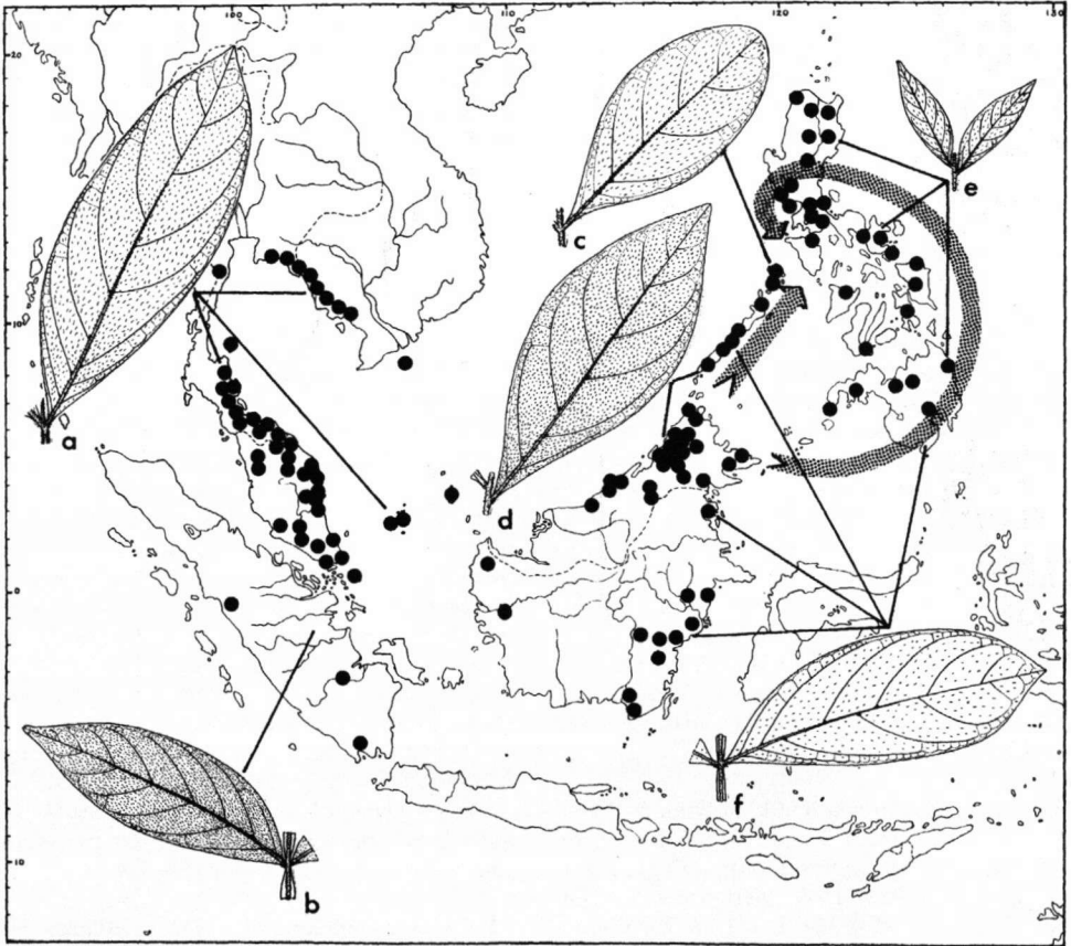
Fig. 42. Guioa pleuroptervis (Blume) Radlk. Distribution map showing two transformation series of leaflets (all c. \cdot 0.7). — a. ' G. pleuroptervis ' form; b. ' G. forbesii ' form; c. ' G. subapiculata ' form; d. ' G. lasiothyrsa ' form; e. ' G. aptera ' form; f. ' G. pleuroptervis ' form (a: Davidson 1325; b: Forbes 2617; c: Merrill 513; d: Elmer 10880; e: Elmer 9315; f: van Niel 4263).
