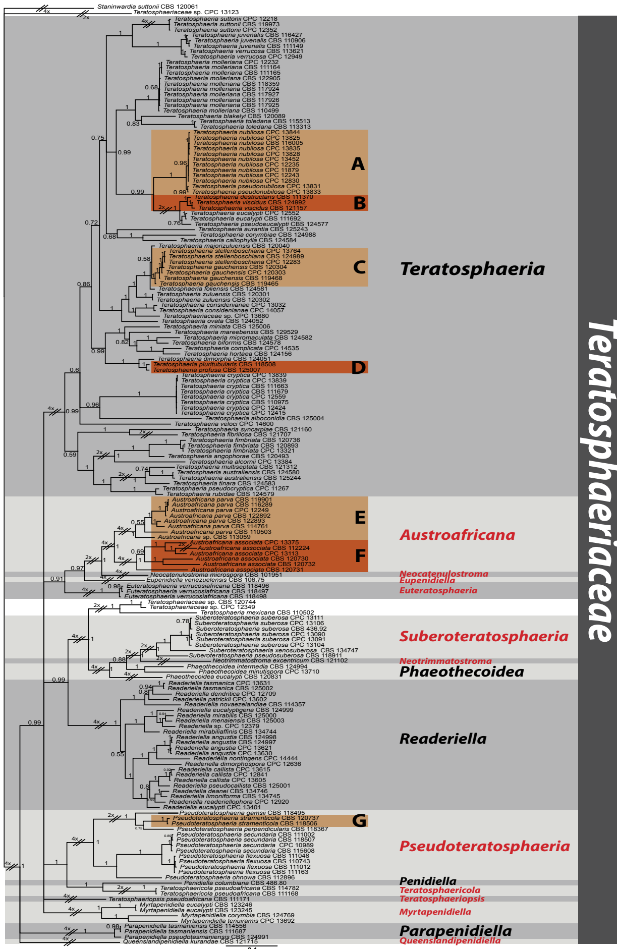
Fig. 1 A Bayesian 50 % majority rule consensus tree based on a combined ITS, LSU, RPB2, EF-1 \alpha and Btub alignment, containing all isolates associated with Teratosphaeria leaf disease of Eucalyptus available at the CBS. Bayesian posterior probabilities support values for the respective nodes are displayed in the tree. The tree was rooted to Staninwardia suttonii . The scale bar indicates 0.1 expected changes per site.
