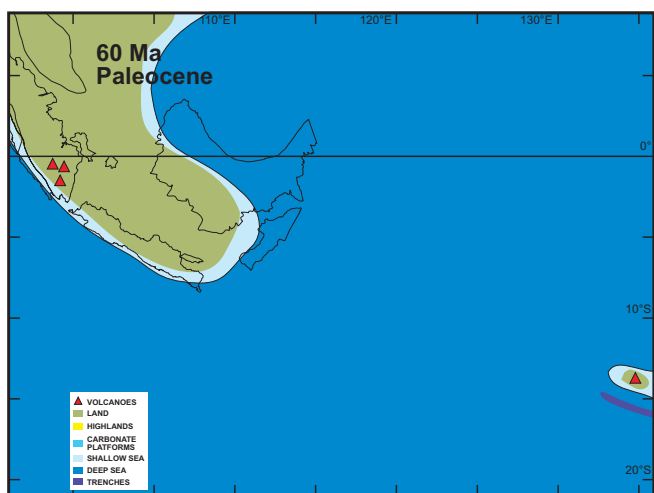
Fig. 7 Postulated distribution of land and sea in the Wallacea region at 60 Ma.
