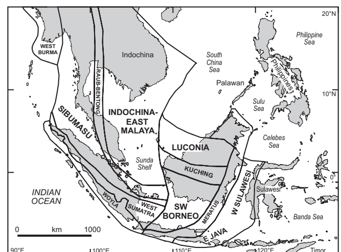
Fig. 4 Late Mesozoic Sundaland. Collision between Sibumasu and East Malaya–Indochina blocks occurred in the Triassic. Additional crust was added to the Sundaland core largely by later collisions of continental blocks.
