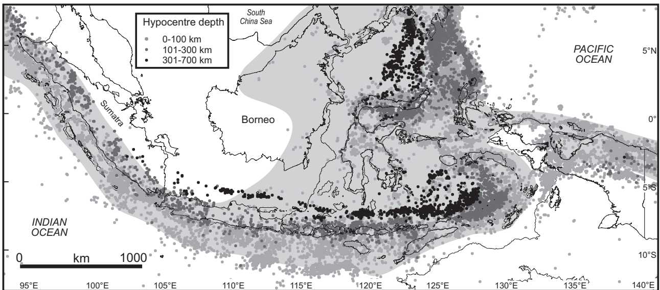
Fig. 2 Seismicity in the circum-Sundaland region between 1964 and 2000. Bathymetric contours are shown at 200 m. The present-day zone of active deformation is shaded light grey.
