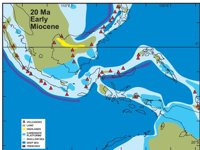
Fig. 11 Postulated distribution of land and sea in the Wallacea region at 20 Ma.
