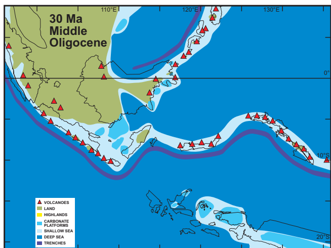
Fig. 9 Postulated distribution of land and sea in the Wallacea region at 30 Ma.
