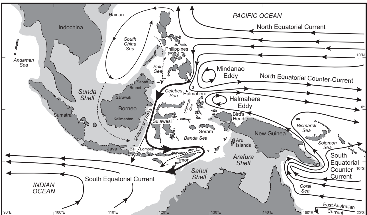
Fig. 15 Major currents in the region of the Indonesian Gateway (modified after Godfrey 1996 and Metzger & Hurlburt 1996) showing the main route of the Indonesian Throughflow from the Pacific Ocean, through the Celebes Sea and Makassar Straits, into the Indian Ocean. There is minor seasonal flow via the South China Sea.
