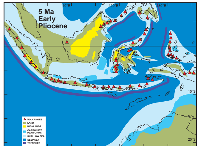
Fig. 14 Postulated distribution of land and sea in the Wallacea region at 5 Ma.
