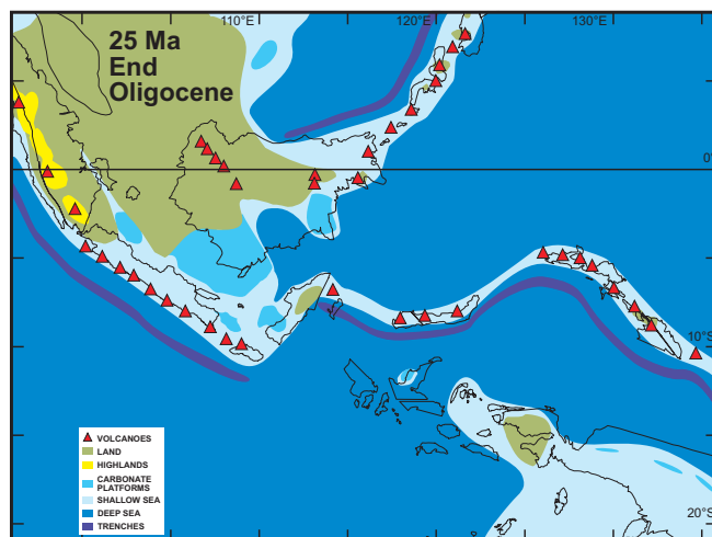
Fig. 10 Postulated distribution of land and sea in the Wallacea region at 25 Ma.
