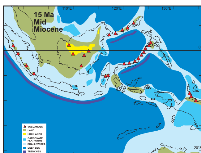
Fig. 12 Postulated distribution of land and sea in the Wallacea region at 15 Ma.
