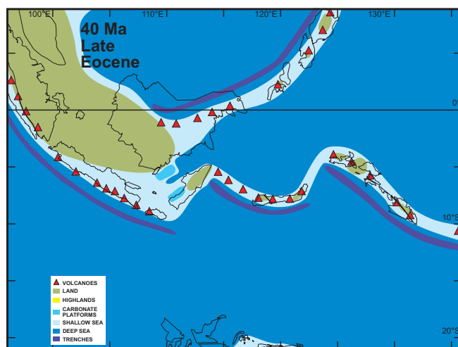
Fig. 8 Postulated distribution of land and sea in the Wallacea region at 40 Ma.
