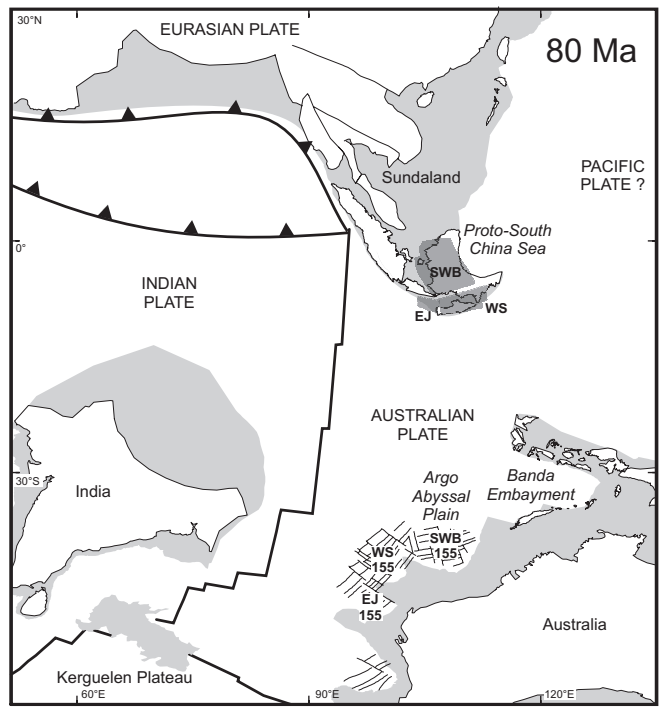
Fig. 6 Reconstruction for the Late Cretaceous after collision of the Southwest Borneo block (SWB), and the later addition of the East Java (EJ) and West Sulawesi (WS) blocks (shaded dark) which terminated subduction beneath Sundaland. The inferred positions of these blocks on the West Australian margin in the Late Jurassic at about 155 Ma are shown by the numbered codes (SWB155, WS155 and EJ155). A transform or very leaky transform spreading centre is inferred to have separated the Indian and Australian Plates between 80 and 45 Ma as India moved rapidly northwards.
