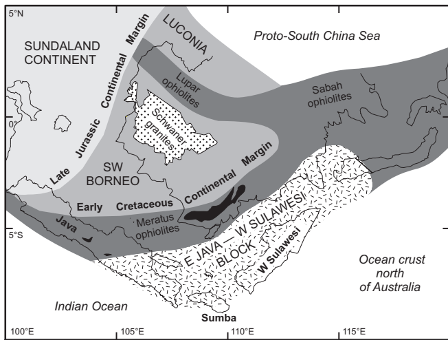
Fig. 5 Inferred positions of the Late Jurassic and the Early Cretaceous Sundaland margin, adapted in part from Hamilton (1979), Parkinson et al. (1998) and Smyth et al. (2007). A suture between pre-Cretaceous Sundaland and the Southwest Borneo block is assumed to be present beneath the Sunda Shelf. Its position is uncertain. The extent and boundaries of the Cathaysian Luconia block are also uncertain. The youngest Cretaceous suture runs from Java and through the Meratus Mountains of Southeast Borneo and to the south and east of this is a continental fragment derived from western Australia (Smyth et al. 2007).
