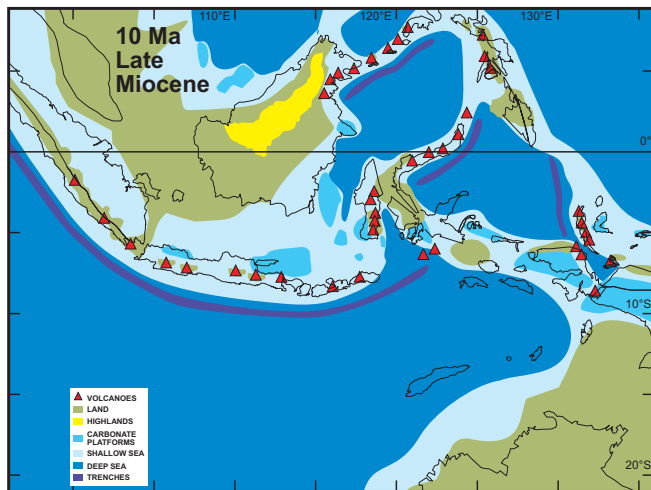
Fig. 13 Postulated distribution of land and sea in the Wallacea region at 10 Ma.
