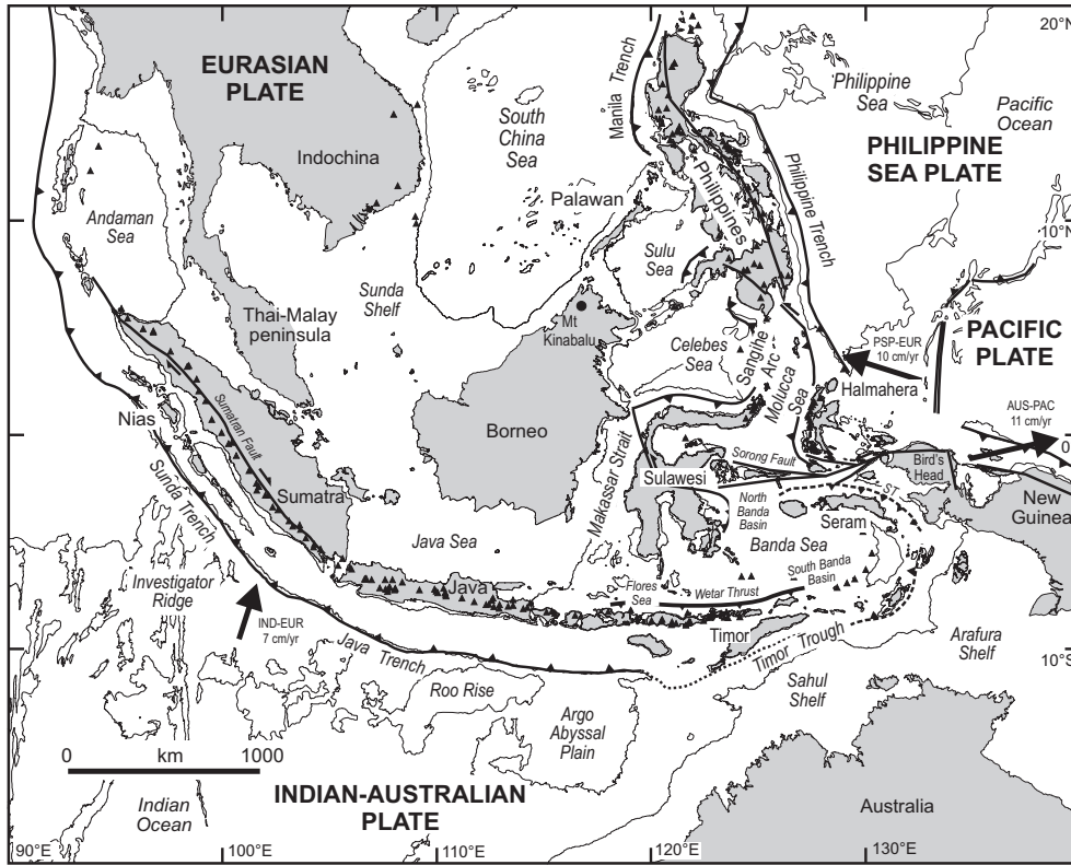
Fig. 1 Geography of Southeast Asia and surrounding regions showing present-day tectonic boundaries and volcanic activity. Bathymetric contours at 200 m and 5 000 m. Heavy arrows show plate convergence vectors for the Indian Plate (IND-EUR), and the Philippine Sea Plate (PSP-EUR) relative to Eurasia, and the Australian Plate relative to the Pacific Plate (AUS-PAC). There is little thrusting at the Timor Trough. The Seram Trough (ST) and Flores-Wetar Thrusts are the sites of active thrusting.
